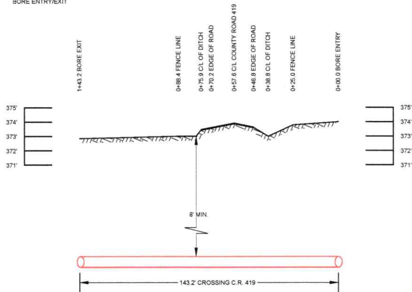
PLAN AND PROFILE OF A PROPOSED PIPELINE CROSSING UNDER COUNTY ROAD 419 ATASCOSA COUNTY, TEXAS
