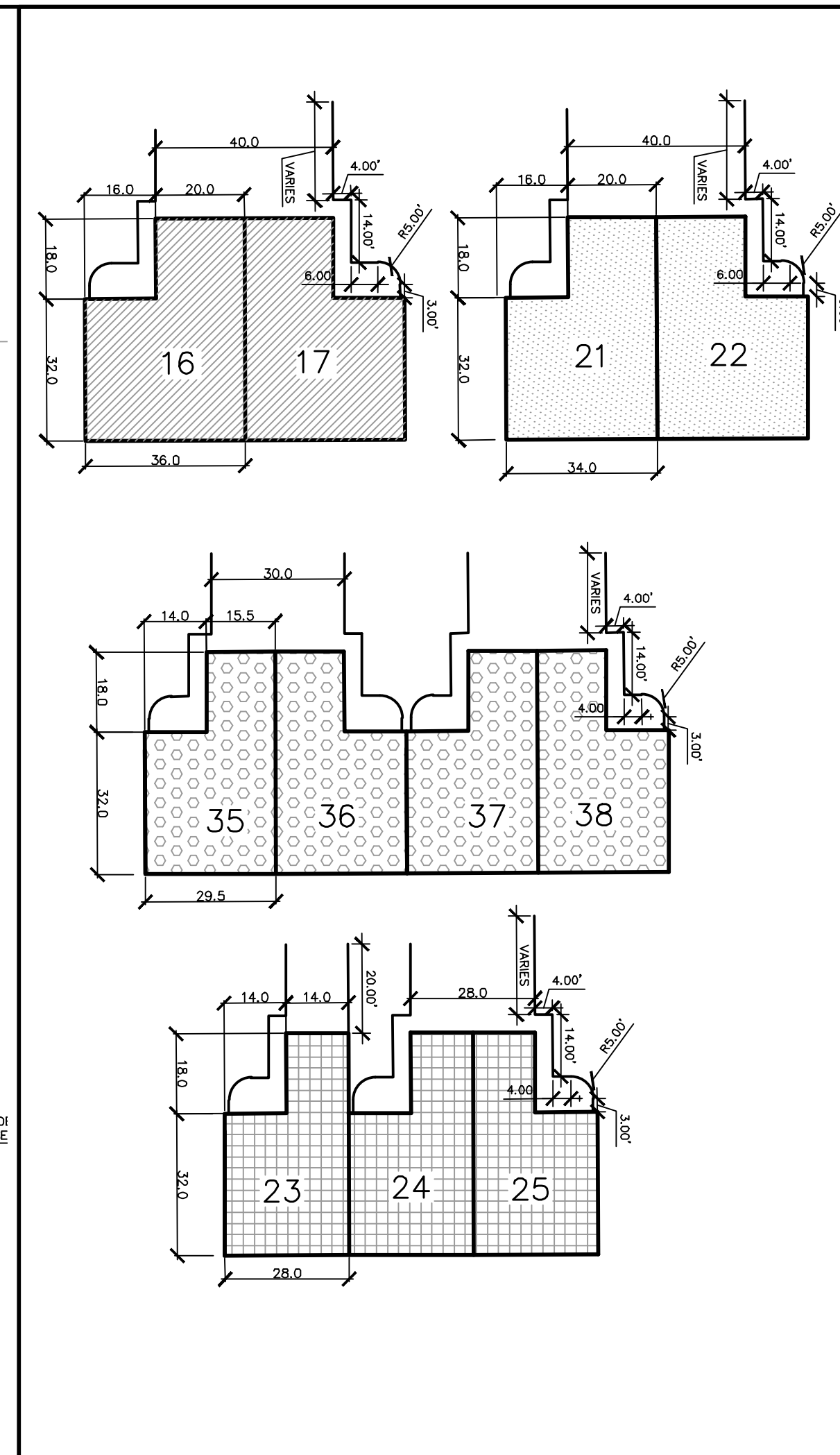
TYPICAL DRIVEWAY & SIDEWALK DETAIL 1" = 30'
