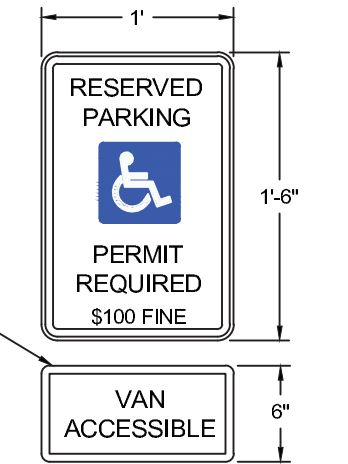
TYPICAL ADA PARKING SIGN SCALE: NTS
