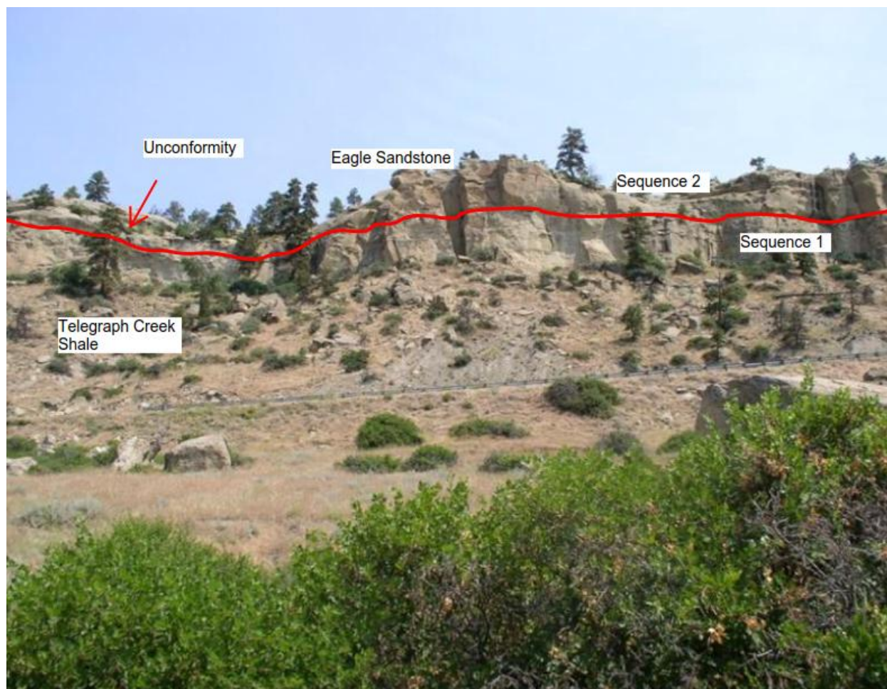
Geologic Stratigraphy at Zimmerman Trail
