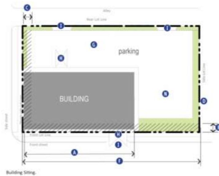
Figure 27-904(10): Building Siting.
