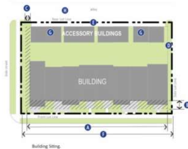
Figure 27-904(1): Building Siting.
