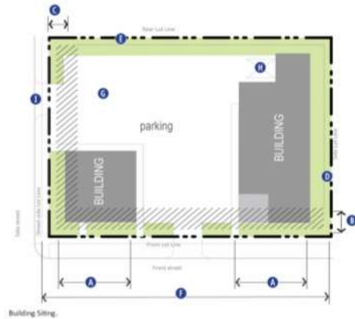
Figure 27-904(13): Building Siting.
