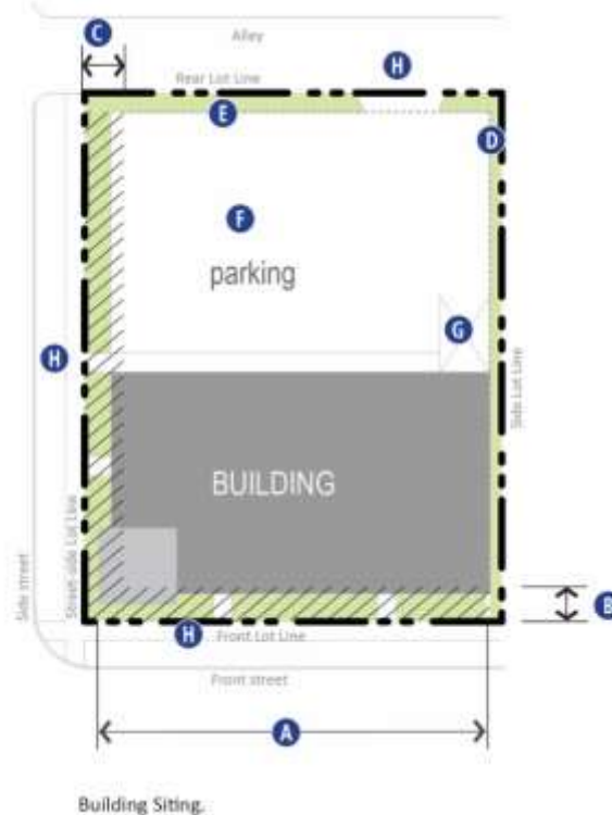
Figure 27-904(4): Building Siting.
