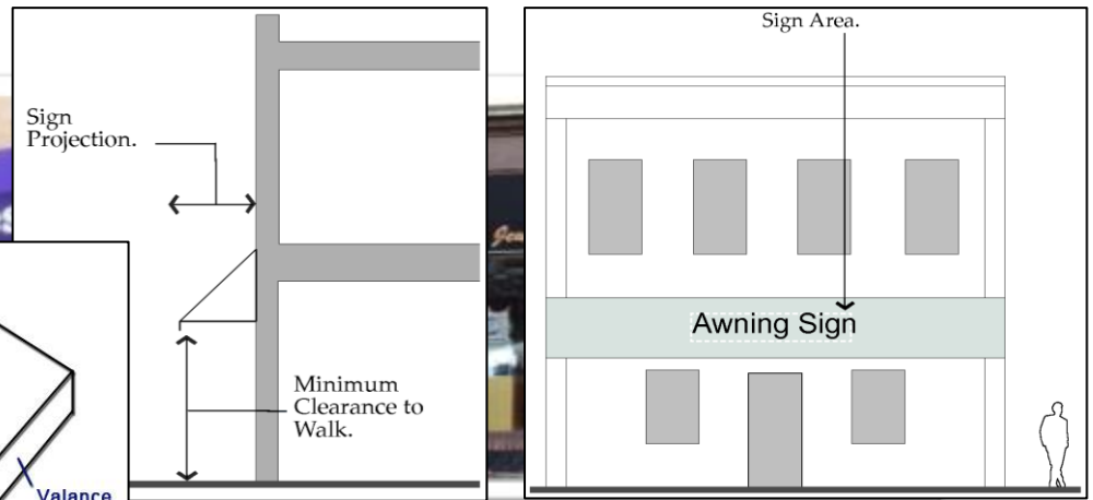
Figure 8: Awning Sign Elements Awning Sign Examples
