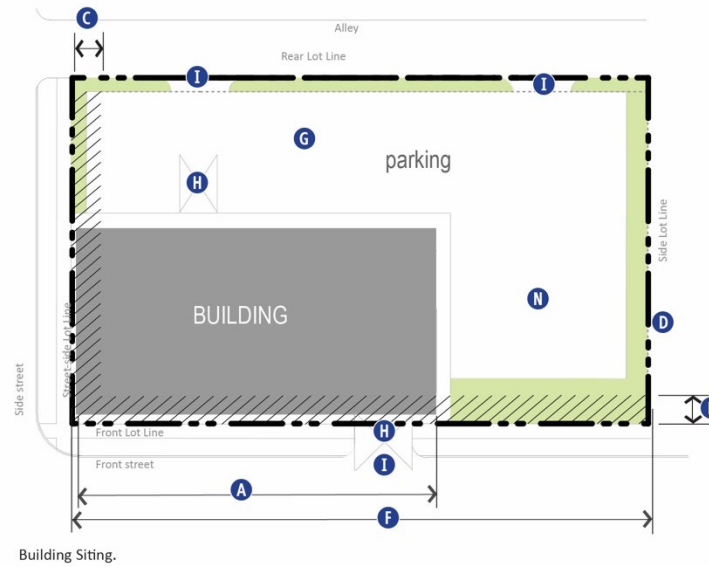
Figure 27-904(10): Building Siting.
