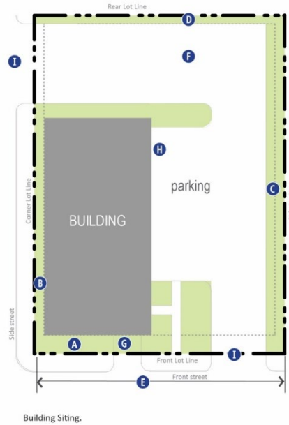
Figure 27-904(16): Building Siting.
