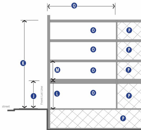
Figure 27-904(10): Building Siting.
