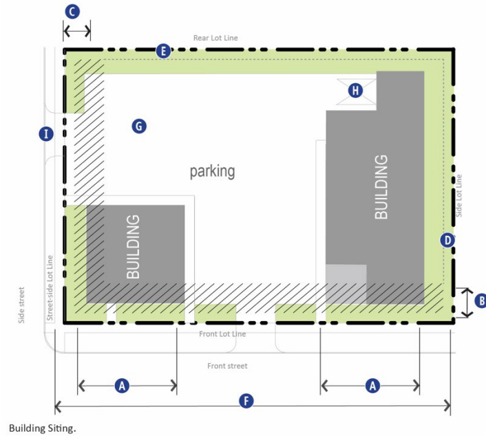
Figure 27-904(13): Building Siting.
