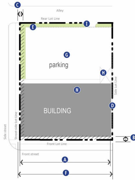
Building Siting.
