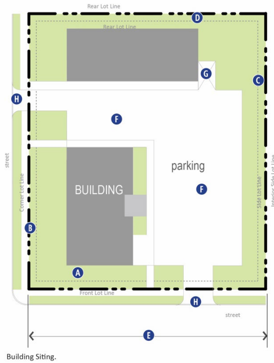
Figure 27-904(19): Building Siting.
