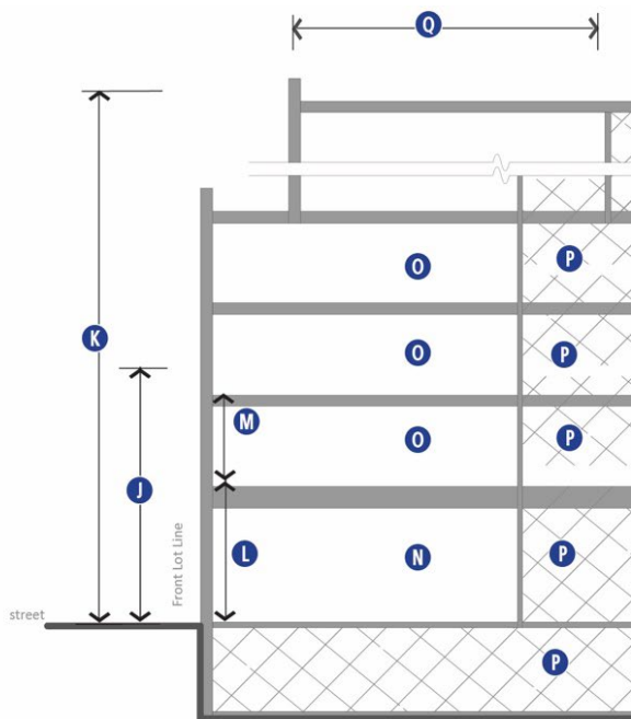
Figure 27-904(7): Building Siting.
