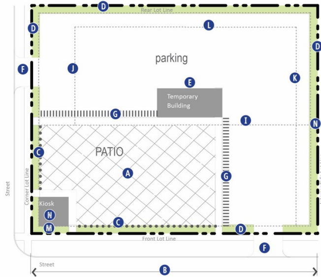
Figure 27-904(22): Building Siting.
