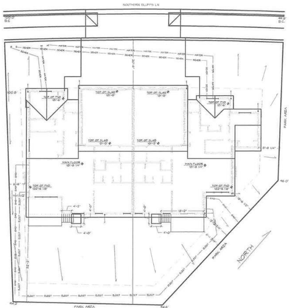
SITE PLAN SCALE: 1"=10'
