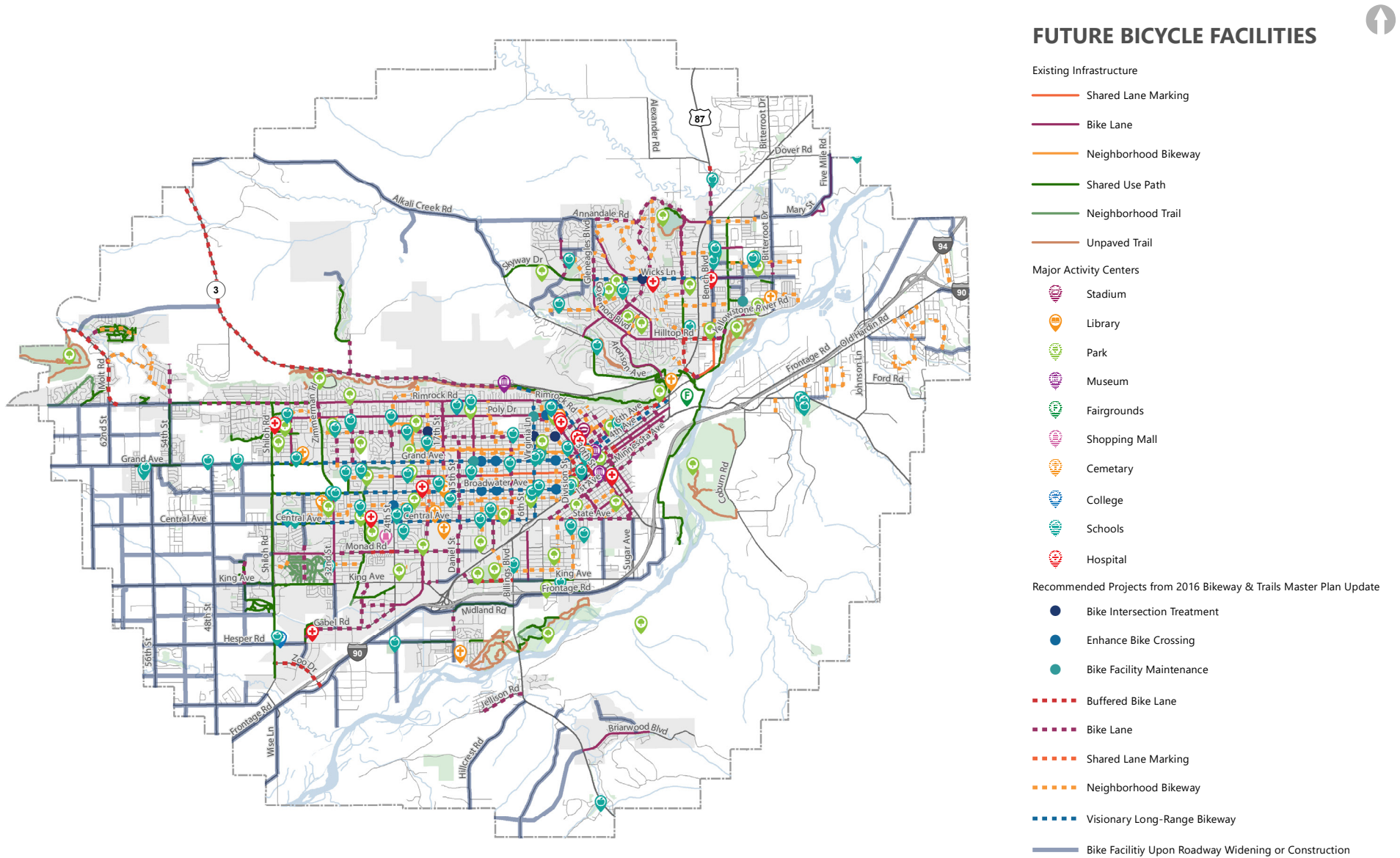
FIGURE 64. FUTURE BICYCLE FACILITIES
