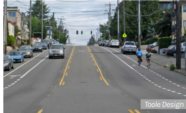
Center turn lane narrowed to provide space for bike lanes
