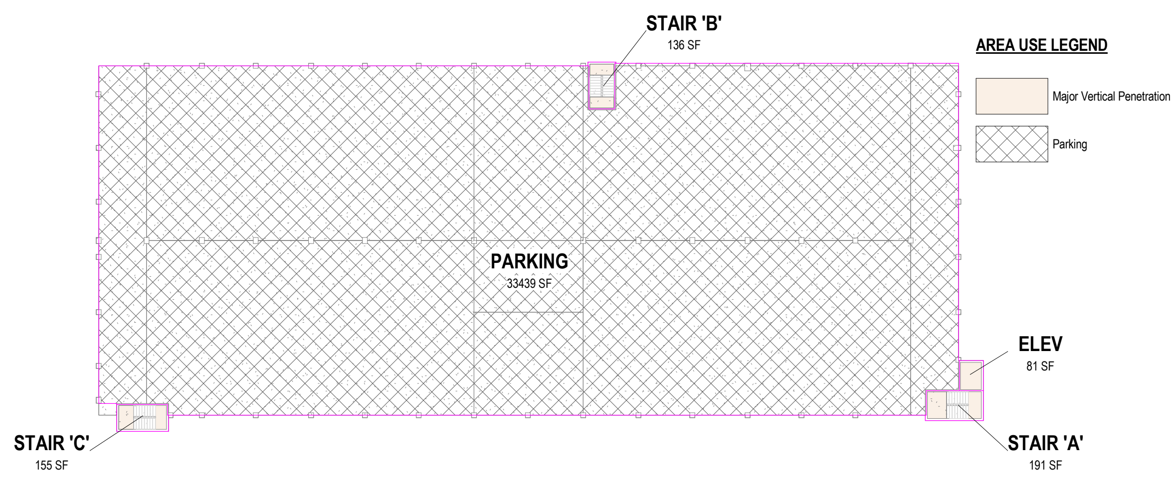
13 LEVEL 5 - AREA USE PLAN 1/32" = 1'-0"
