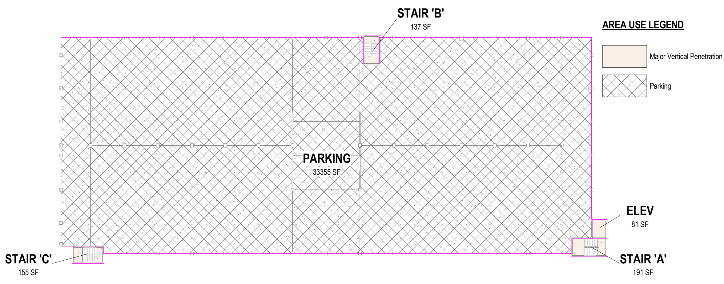
5 LEVEL 1 - AREA USE PLAN 1/16" = 1'-0"
