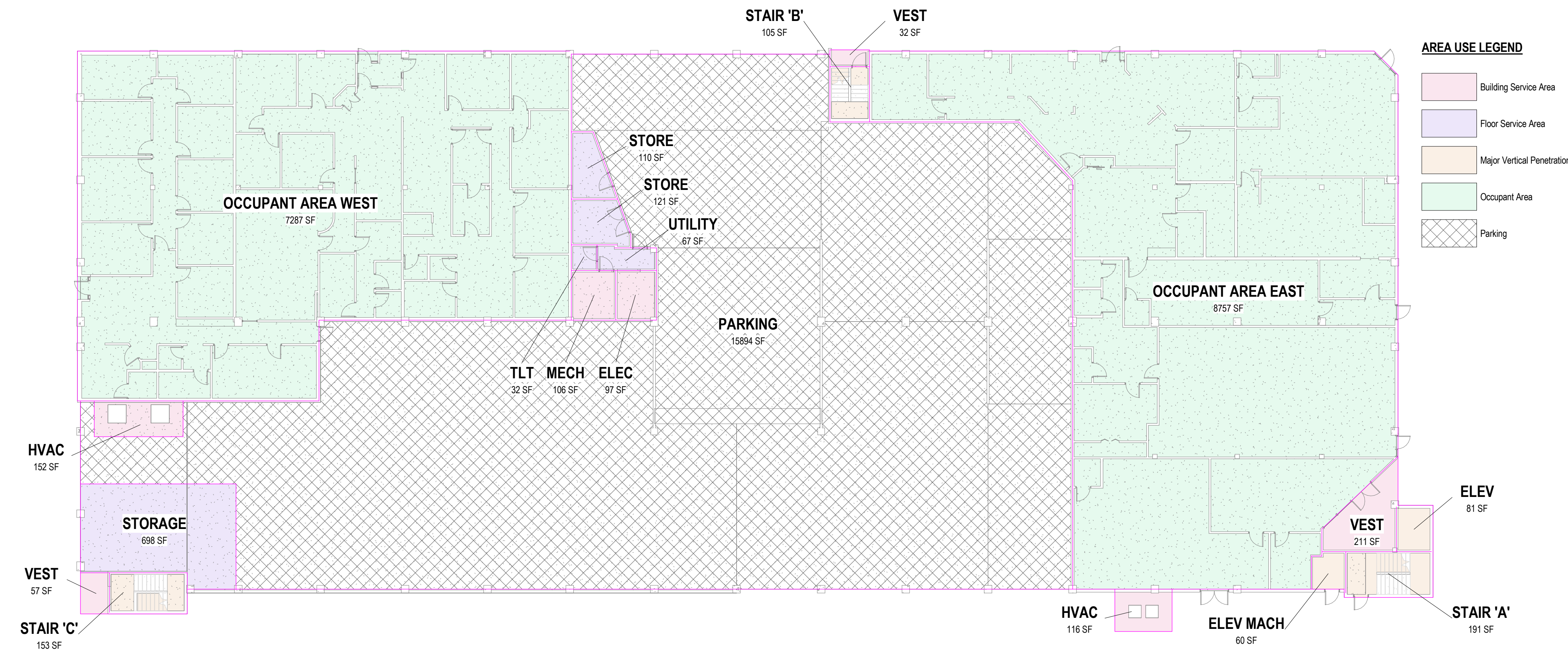
5 LEVEL 1 - AREA USE PLAN 1/16" = 1'-0"
