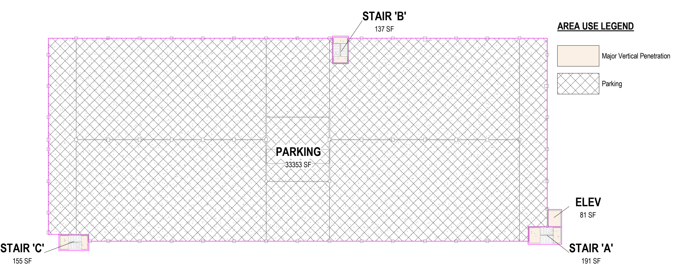
15 LEVEL 3 - AREA USE PLAN 1/32" = 1'-0"
