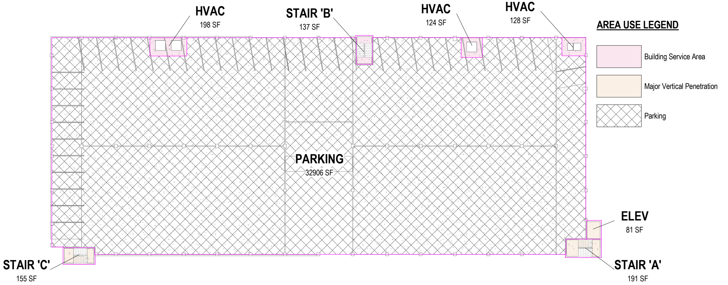
11 LEVEL 2 - AREA USE PLAN 1/32" = 1'-0"
