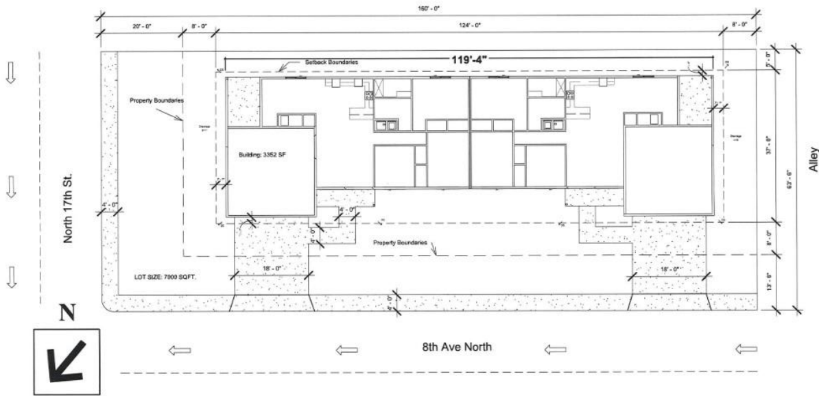
① Site Plan 1/16" = 1'-0"
