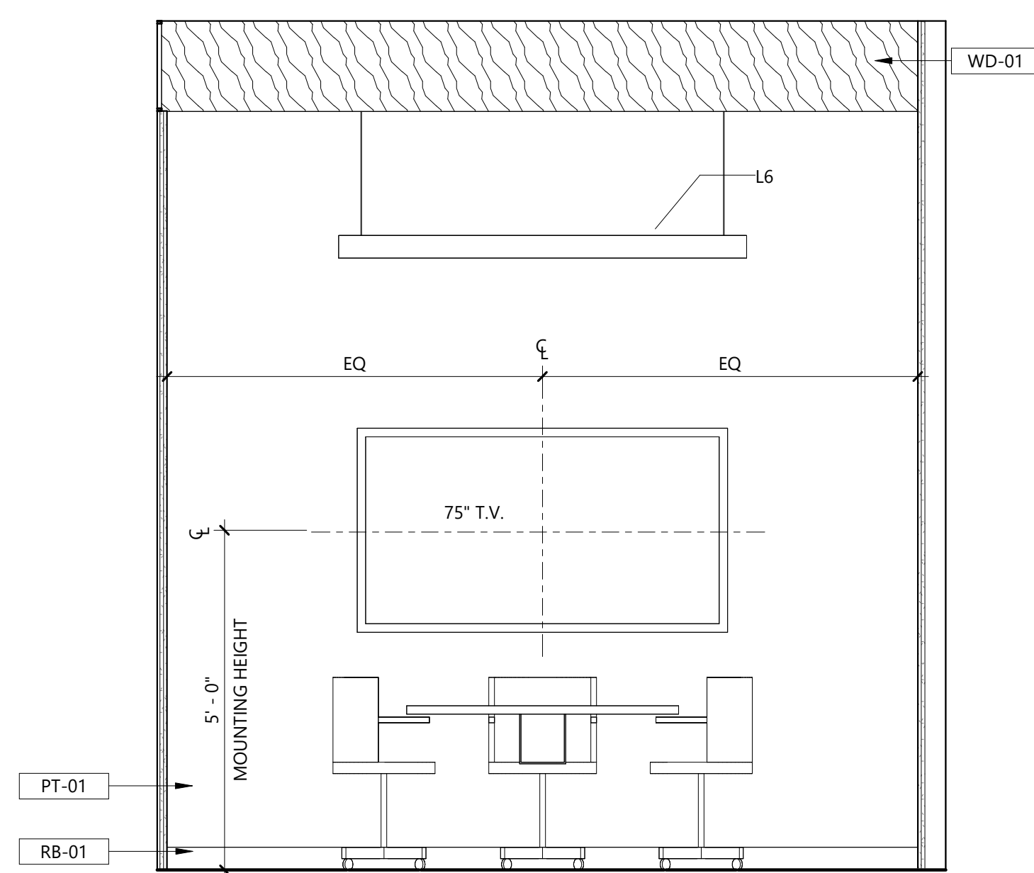
3 CONFERENCE SCALE: 1/2" = 1'-0"
