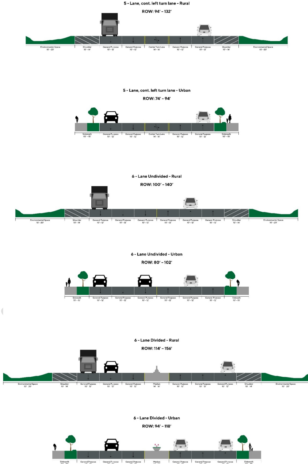
Figure 40. Typical Roadway Cross Sections illustrations
