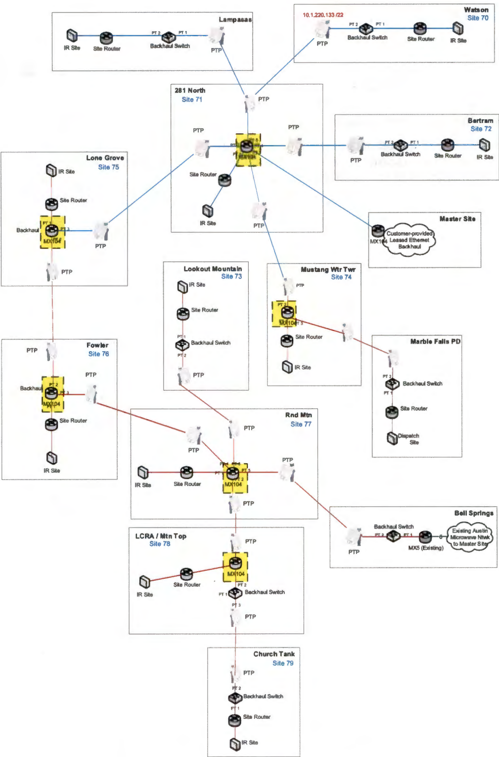
Figure 1-1: Western Counties Network Design
