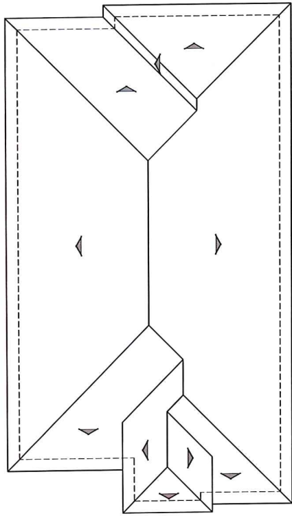
ROOF PLAN C PITCH: 4:12 RAKE: N/A EAVE: 24" ROOF MATERIAL: FLAT CONCRETE TILE
