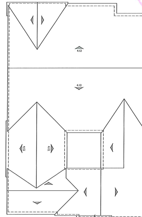
ROOF PLAN
