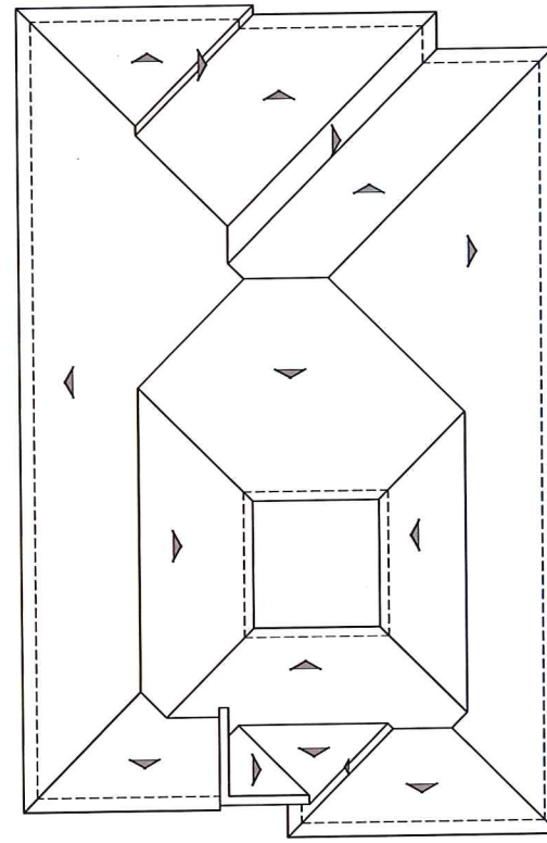
ROOF PLAN
