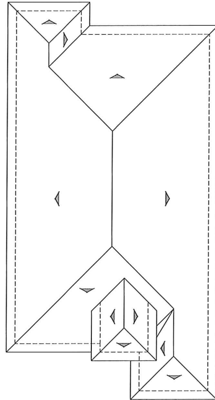
ROOF PLAN PITCH: 4:12 RAKE: N/A EAVE: 24" ROOF MATERIAL: FLAT CONCRETE TILE
