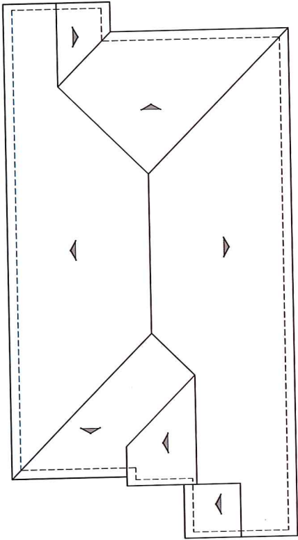
ROOF PLAN A PITCH: 4:12 RAKE: 4° EAVE: 18" ROOF MATERIAL: CONCRETE 'S' TILE
