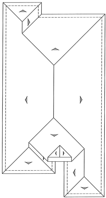
ROOF PLAN PITCH: 4:12 RAKE: N/A EAVE: 18" ROOF MATERIAL: FLAT CONCRETE TILE
