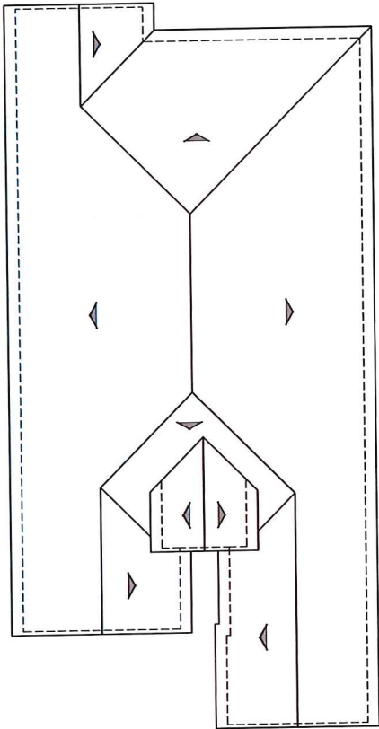
ROOF PLAN A PITCH: 4:12 RAKE: 4" EAVE: 18" ROOF MATERIAL: CONCRETE 'S' TILE
