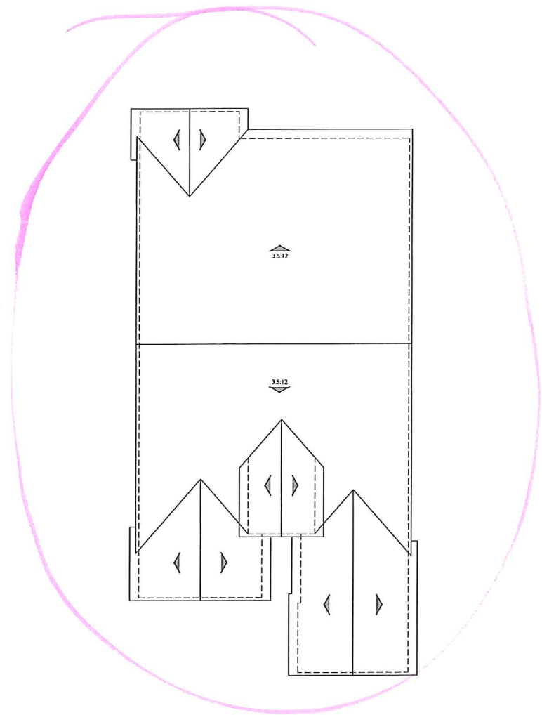
ROOF PLAN
