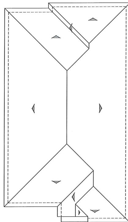
ROOF PLAN
