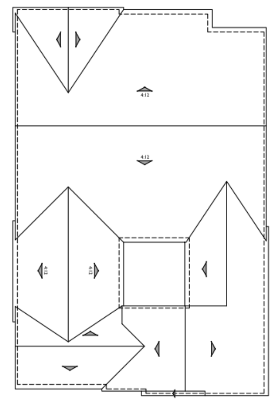
ROOF PLAN D PITCH: 6:12 RAKE: 6" EAVE: 12" ROOF MATERIAL: FLAT CONCRETE TILE
