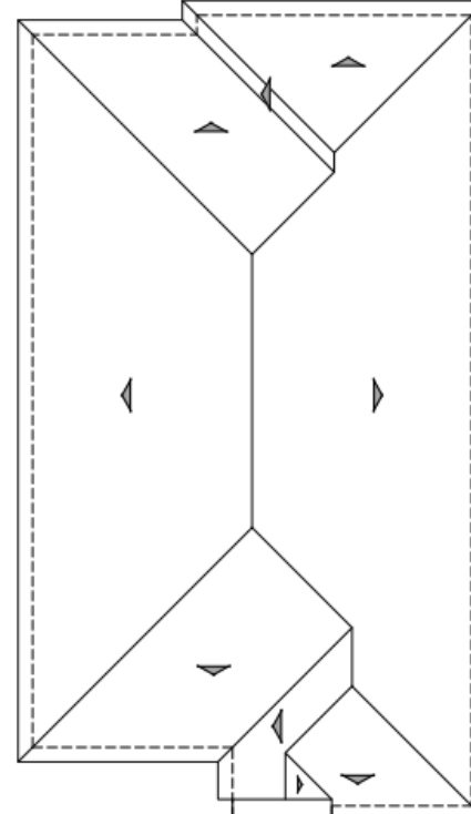
ROOF PLAN B PITCH: 4:12 RAKE: N/A EAVE: 18" ROOF MATERIAL: FLAT CONCRETE TILE
