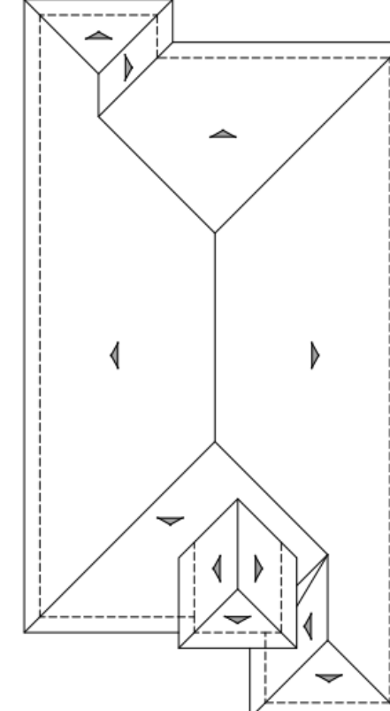
ROOF PLAN C PITCH: 4:12 RAKE: N/A EAVE: 24" ROOF MATERIAL: FLAT CONCRETE TILE
