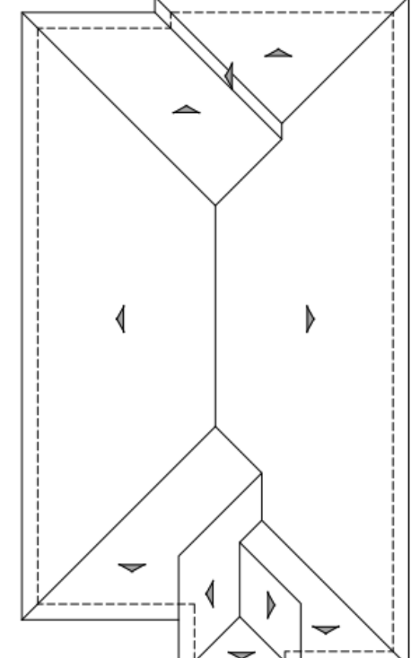
ROOF PLAN C PITCH: 4:12 RAKE: N/A EAVE: 24" ROOF MATERIAL: FLAT CONCRETE TILE
