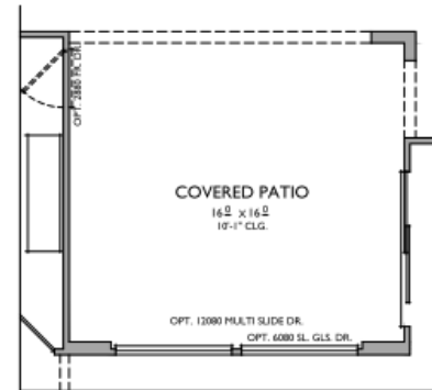
EXTENDED COVERED PATIO +99 SQ. FT.
