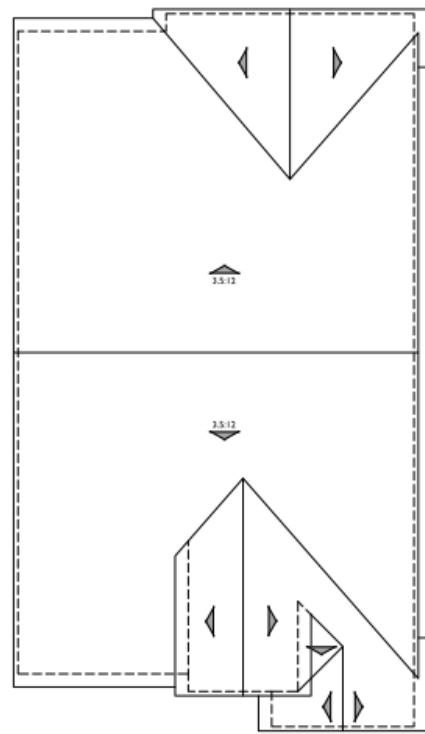
ROOF PLAN A PITCH: 4:12 RAKE: 6" EAVE: 18" ROOF MATERIAL: CONCRETE S TILE
