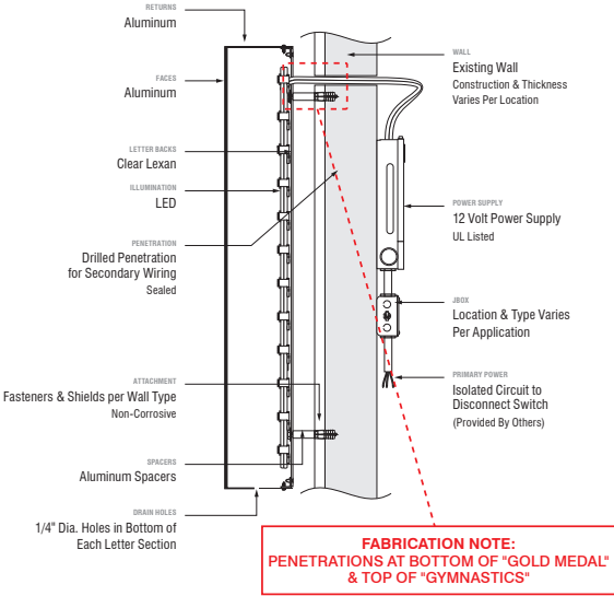
B Section Detail - Typical Reverse Pan Channel Letter / LED Halo-Illuminated
