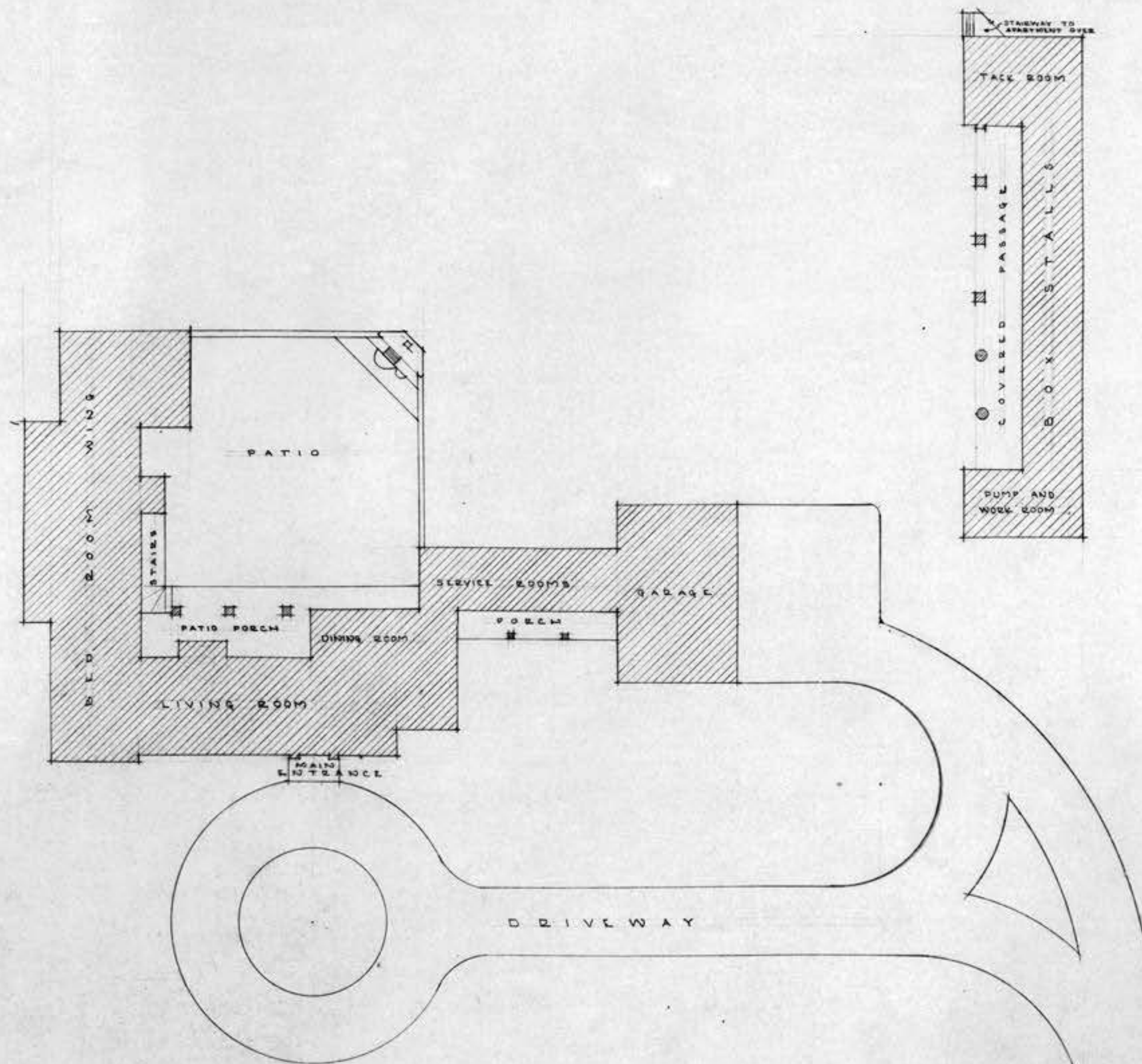
PLOT PLAN SCALE 1/8" = 1'-0"
