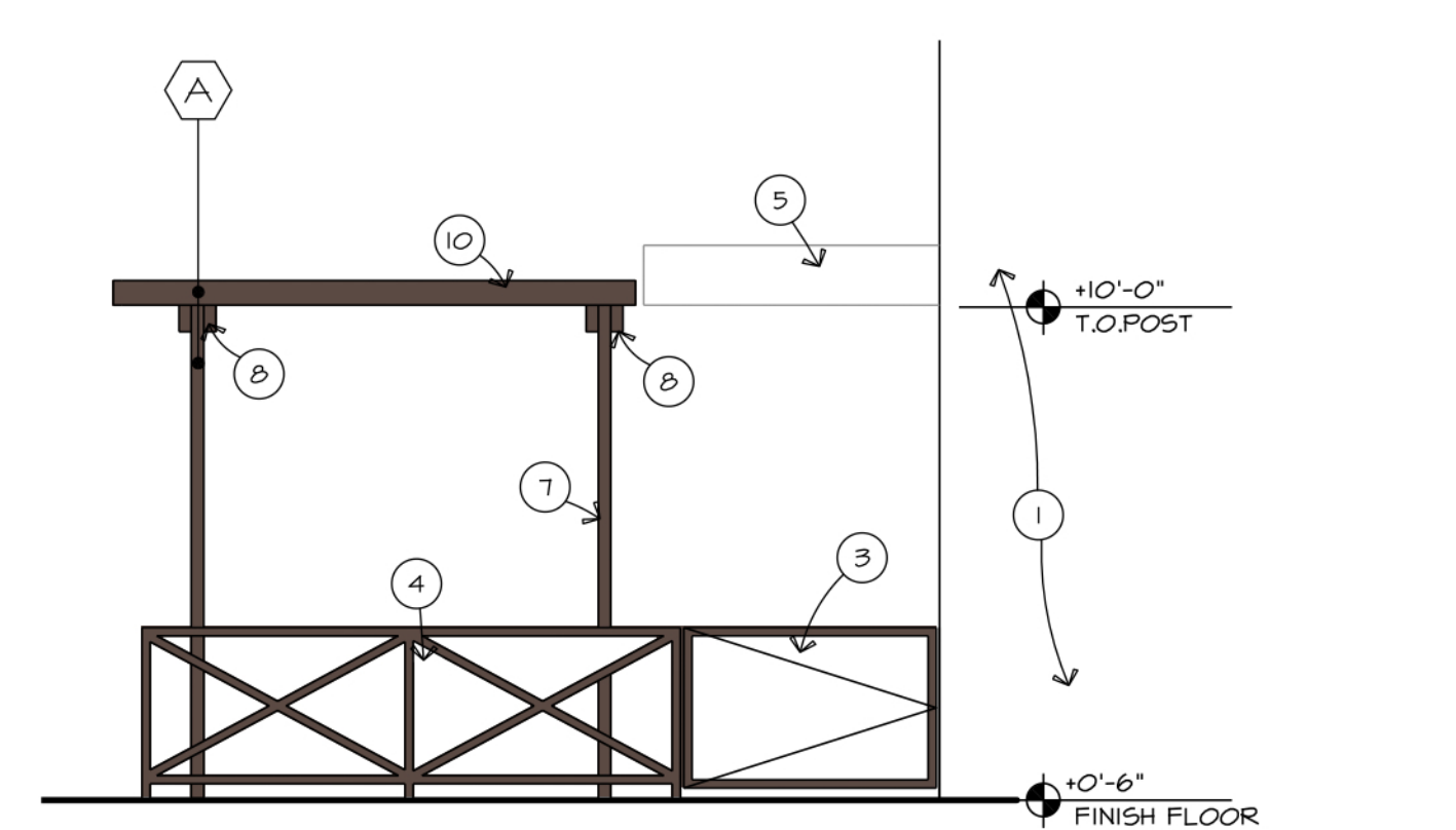
NORTH ELEVATION
