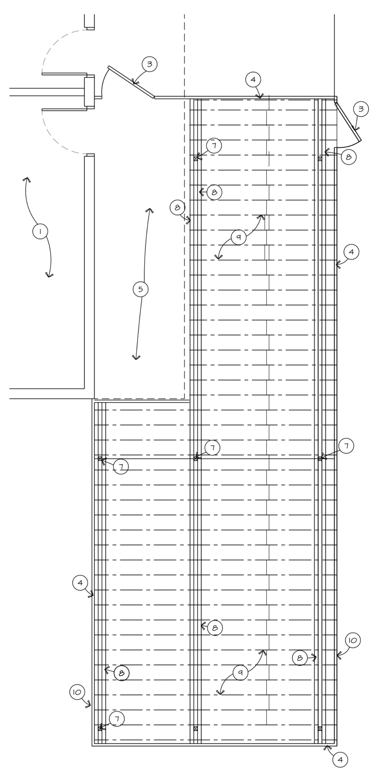
ENLARGED PATIO FRAMING PLAN
