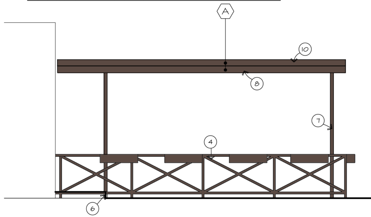
WEST ELEVATION
