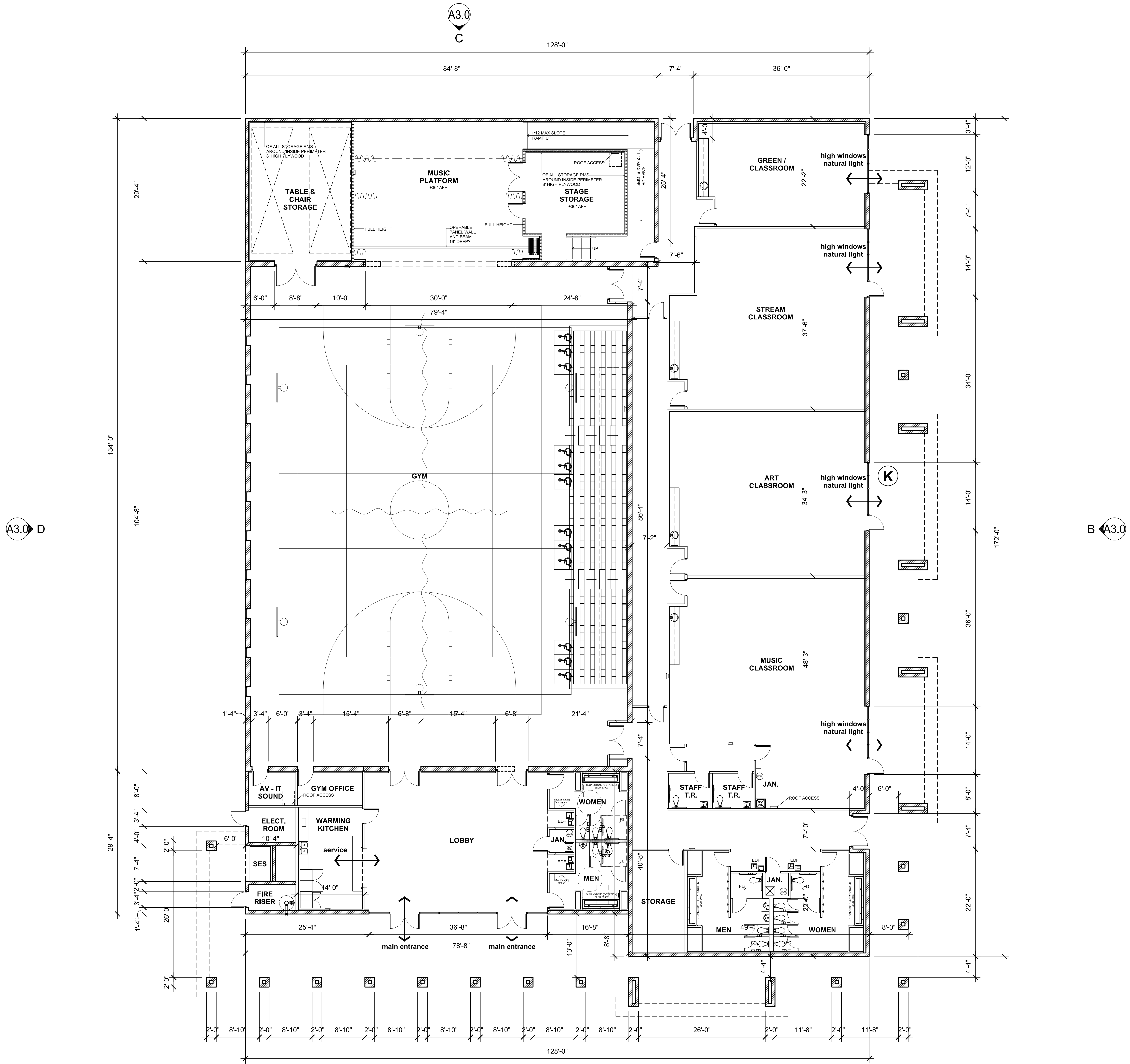
FLOOR PLAN SCALE: 1/8" = 1'-0" 21,300 sf (gross floor area)
