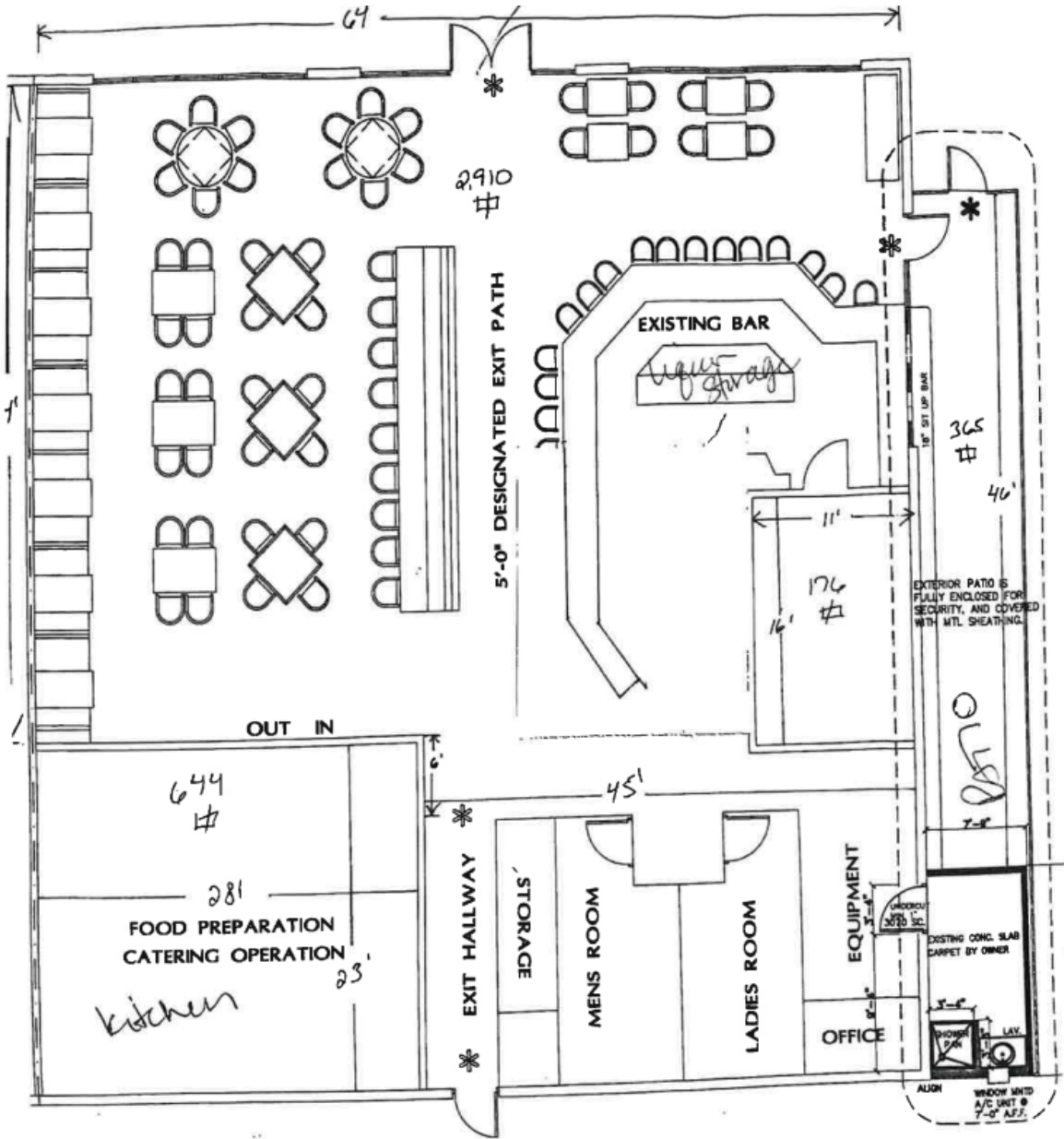
FLOOR PLAN
