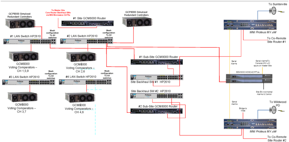
Figure 1-5: Basic Diagram of a Typical ASTRO 25 Simulcast Prime Site
