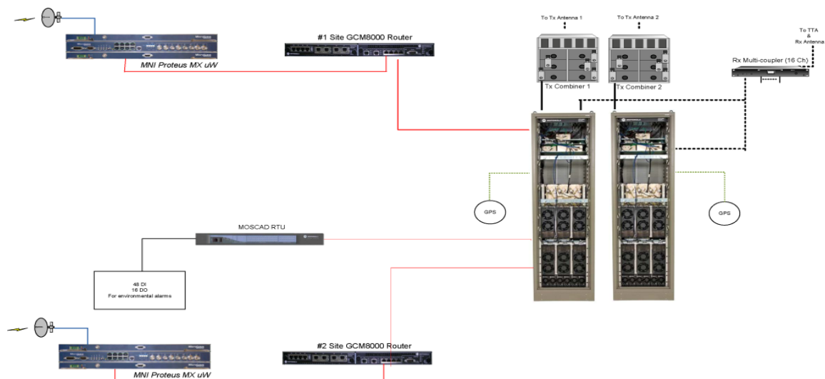
Figure 1-6: Basic Diagram of a Typical ASTRO 25 Simulcast Remote Site
