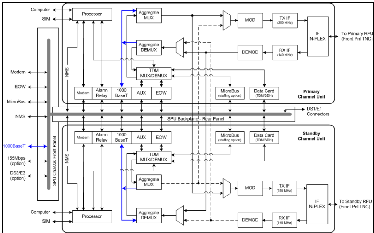
Figure 5 Proteus MX 1+1 Signal Processing Unit Block Diagram
