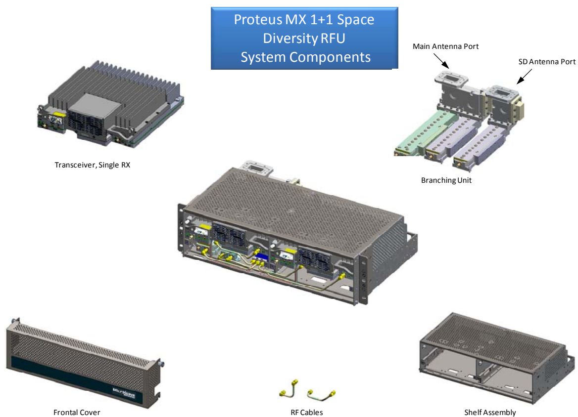
Figure 4 Proteus MX 1+1 Space Diversity Hot Standby Indoor RF Unit
