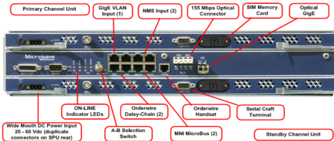
Figure 2- Proteus MX 2+0 Signal Processing Unit - Front
