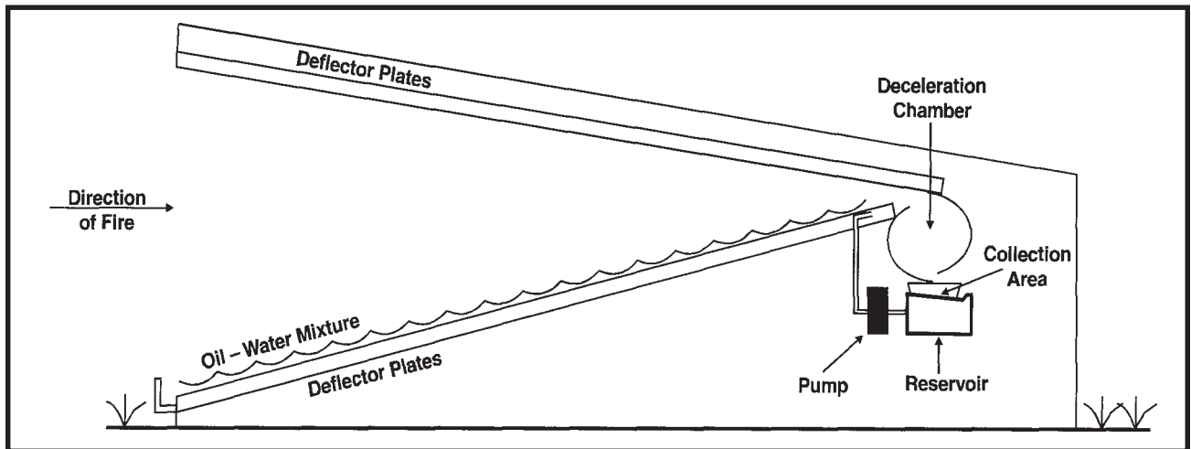
Wet Passive Trap (Adapted from: Bullet Trap Feasibility Assessment and Implementation Plan: Technology Identification Final Report , U.S. Army Environmental Center, March 1996)
