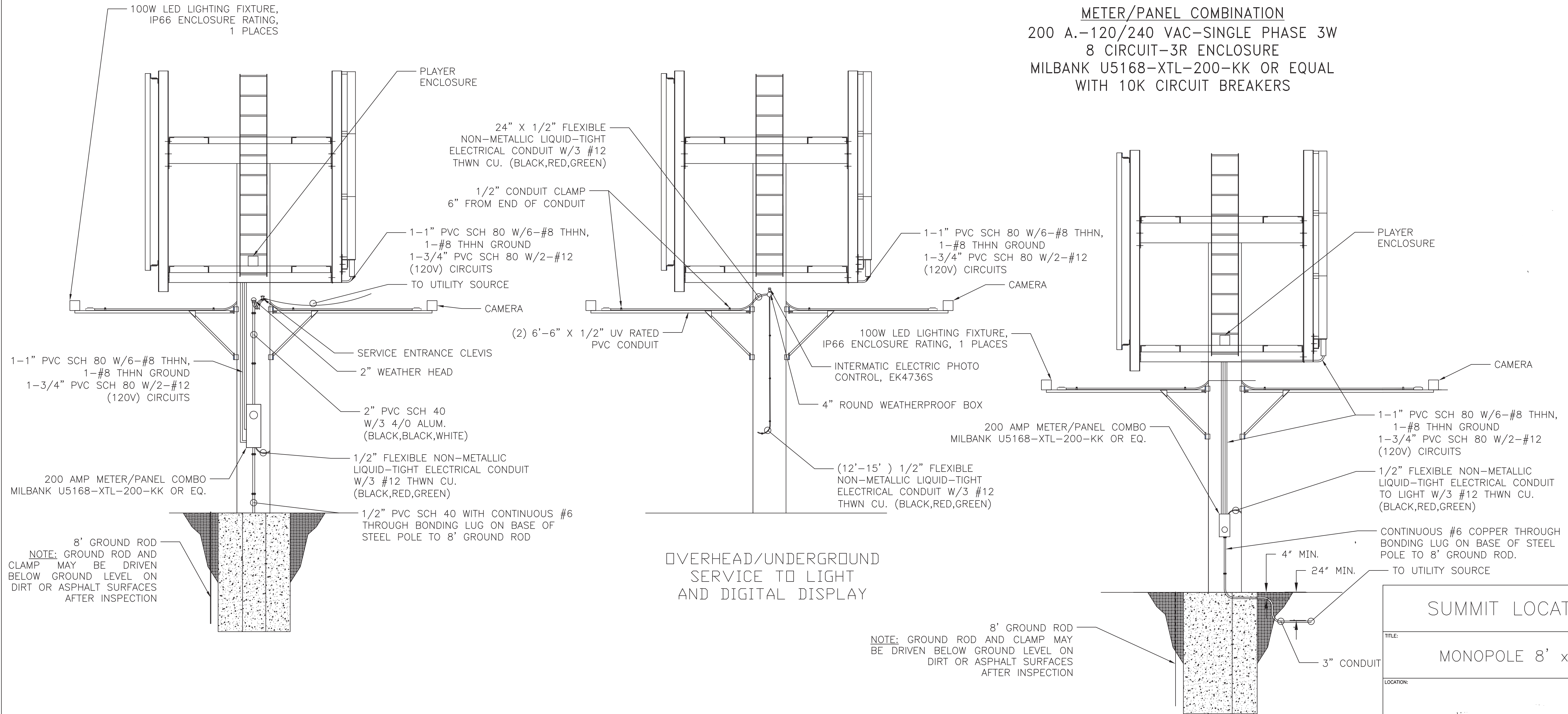
OVERHEAD SERVICE ENTRANCE
