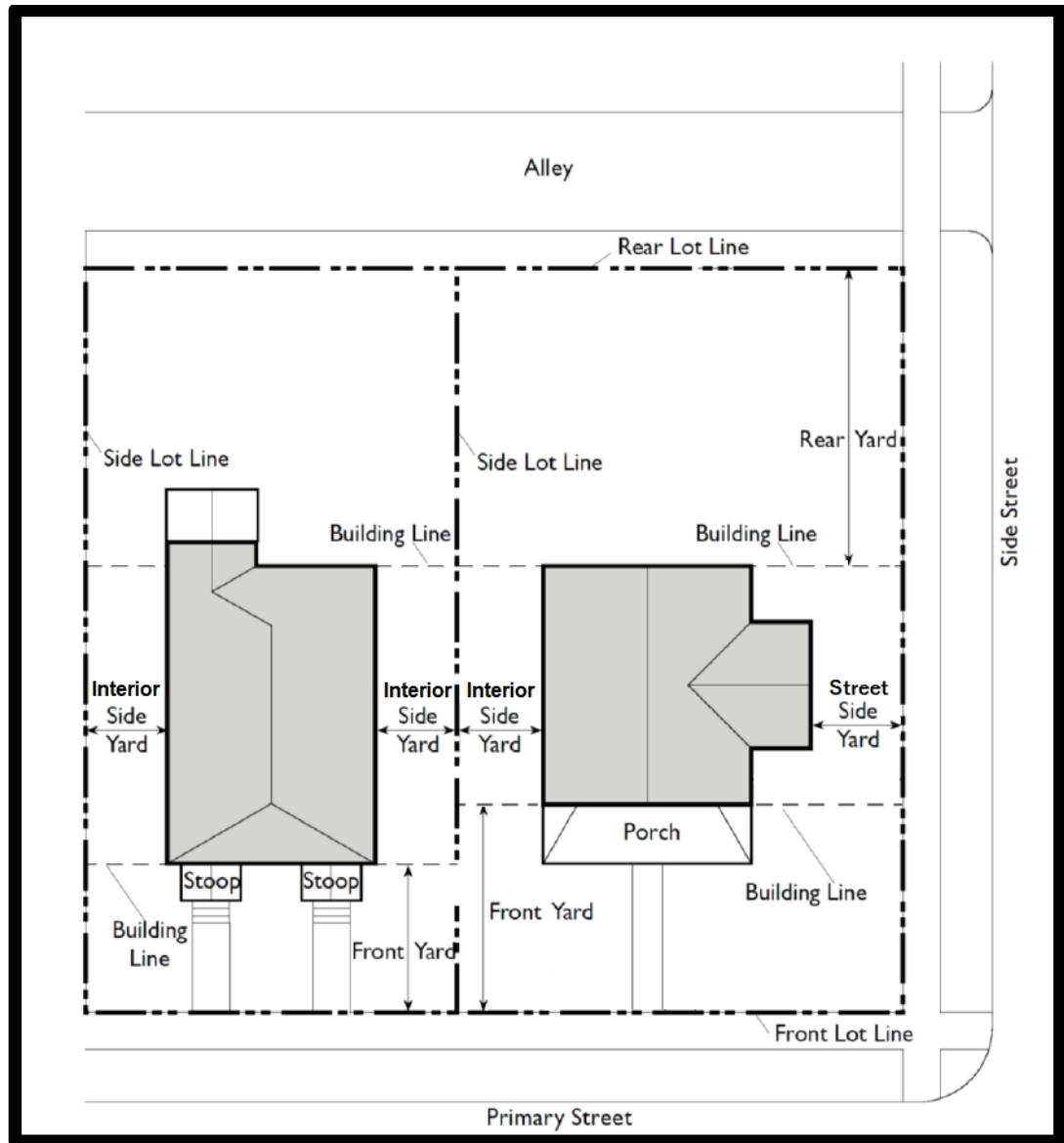
Figure 10-80.20.250. Yards.
