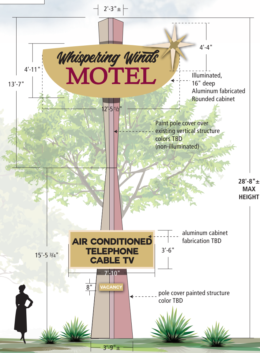
Monument Refurb. Elevation | Scale: 3/16"=1'-0"
