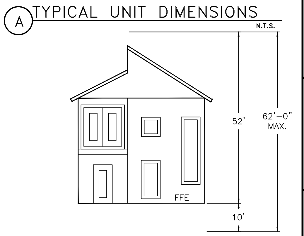
A TYPICAL UNIT DIMENSIONS B TYPICAL BUILDING ELEVATION
