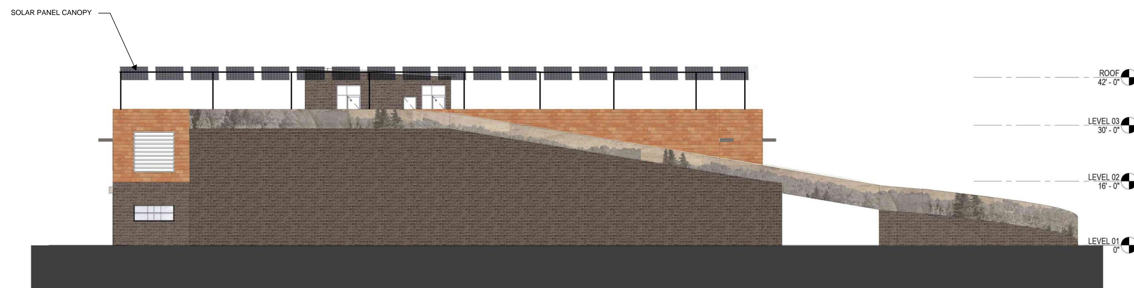
A5 WEST ELEVATION - PHASE 01 1/16" = 1'-0"
