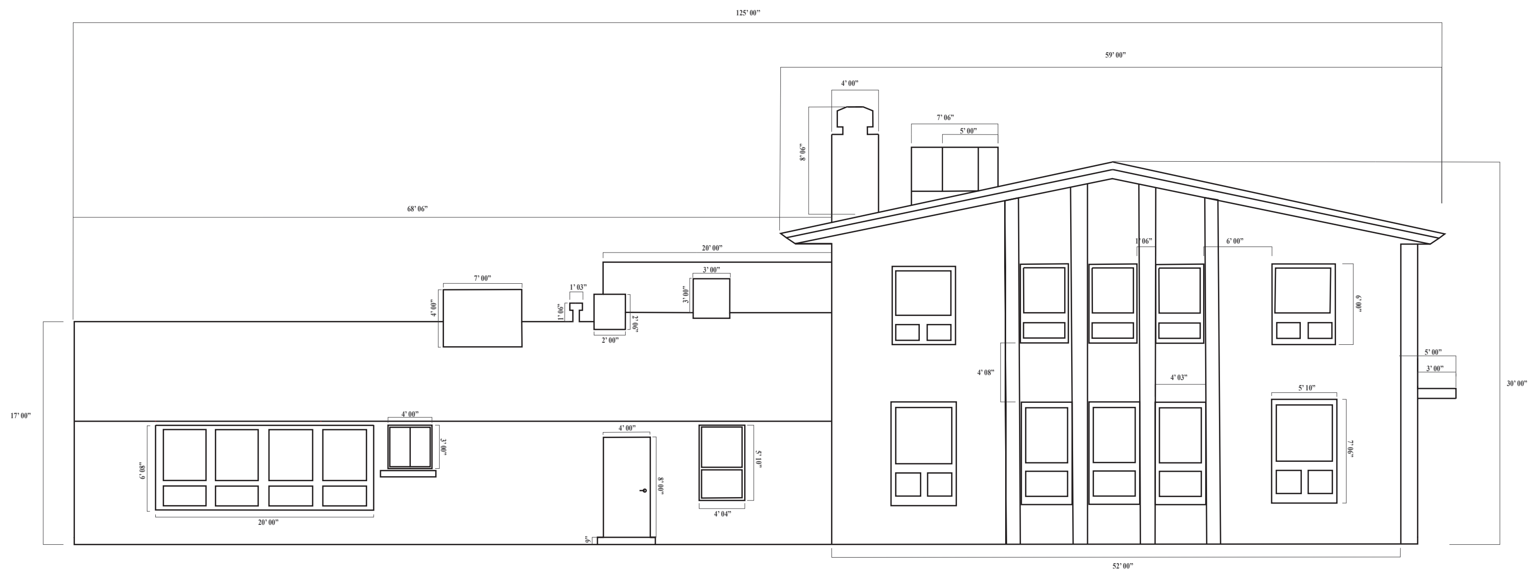
North Elevation of 18 W Birch 1:96 Scale
