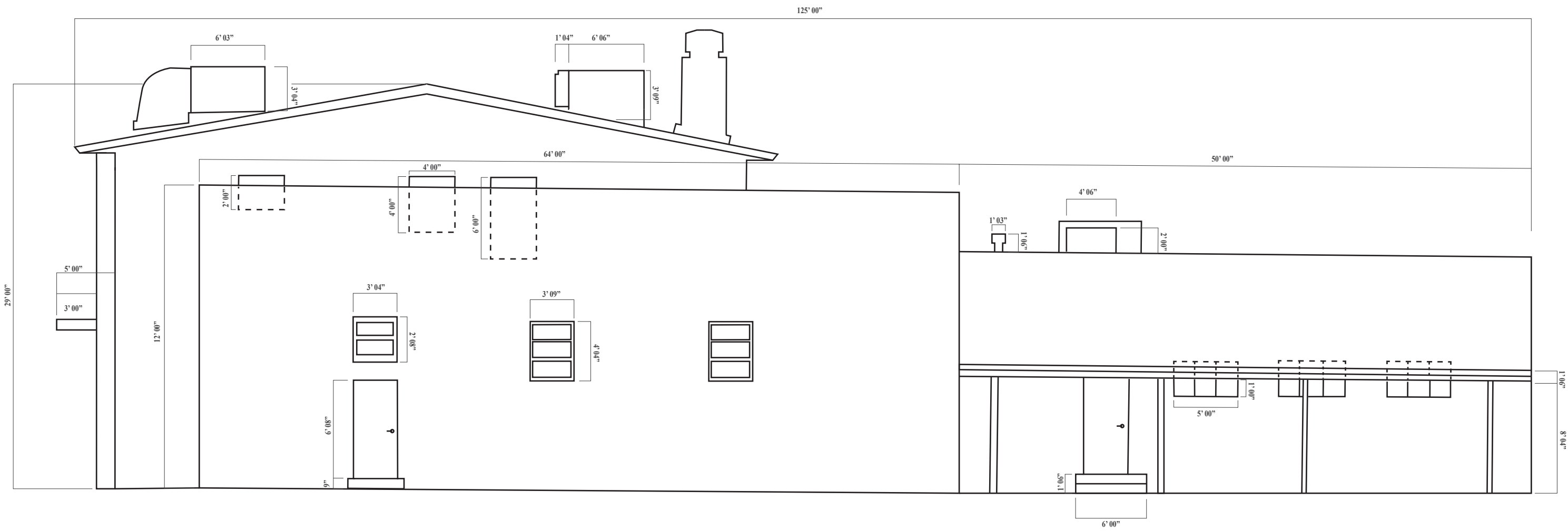
South Elevation of 18 W Birch 1:96 Scale
