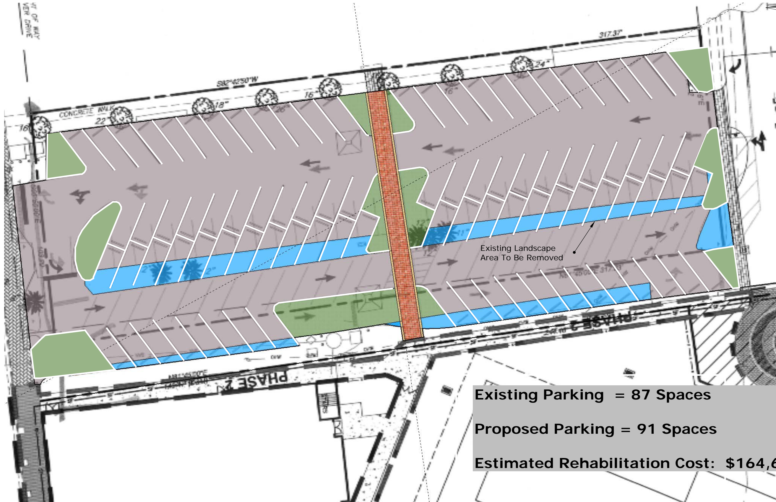
Melody Lane Parking Area - Rehabilitation
