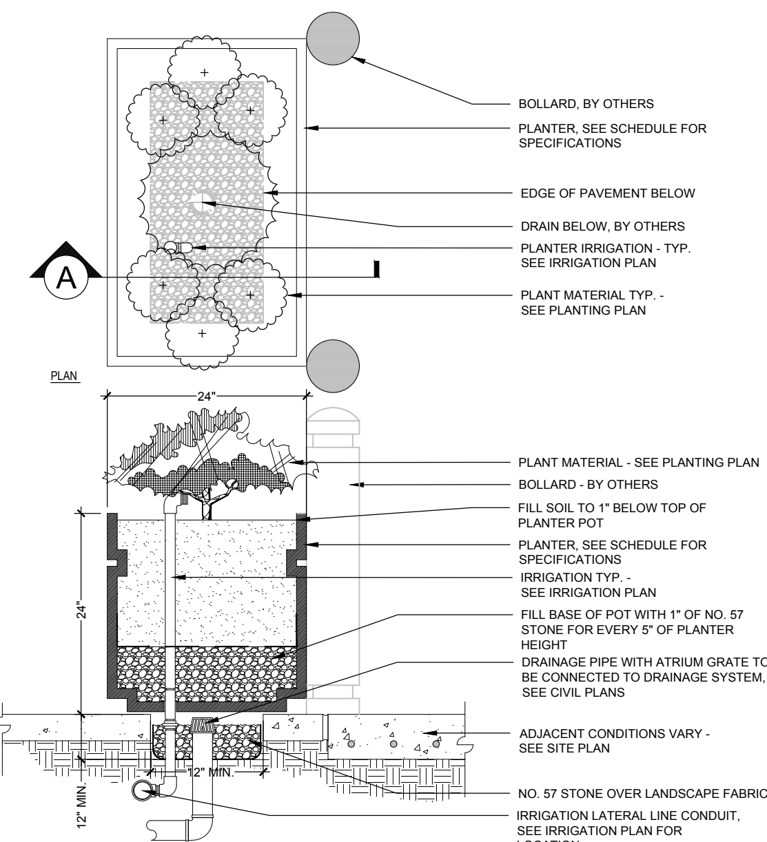
6 TYPICAL RAISED PLANTER DETAIL SCALE: NTS
