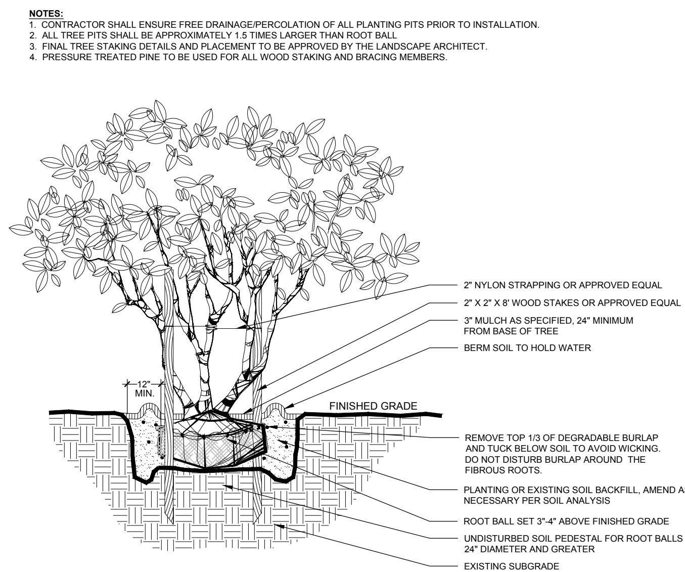
5 MULTI-STEM UNDERSTORY TREE SCALE: NTS
