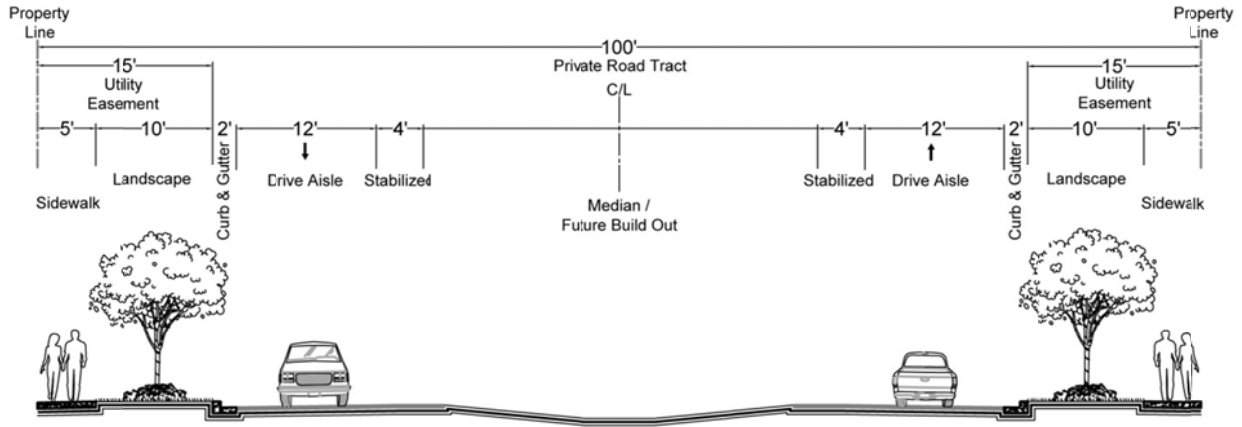
CENTER ROAD (PHASE 1) 100' PRIVATE ROAD TRACT n.t.s.
