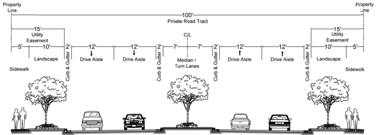
CENTER ROAD (PHASE 1) 100' PRIVATE ROAD TRACT n.t.s.
