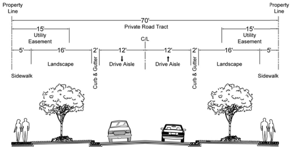
WESTERN ACCESS RD. (NORTHERN SECTION) 70' PRIVATE ROAD TRACT n.t.s.
