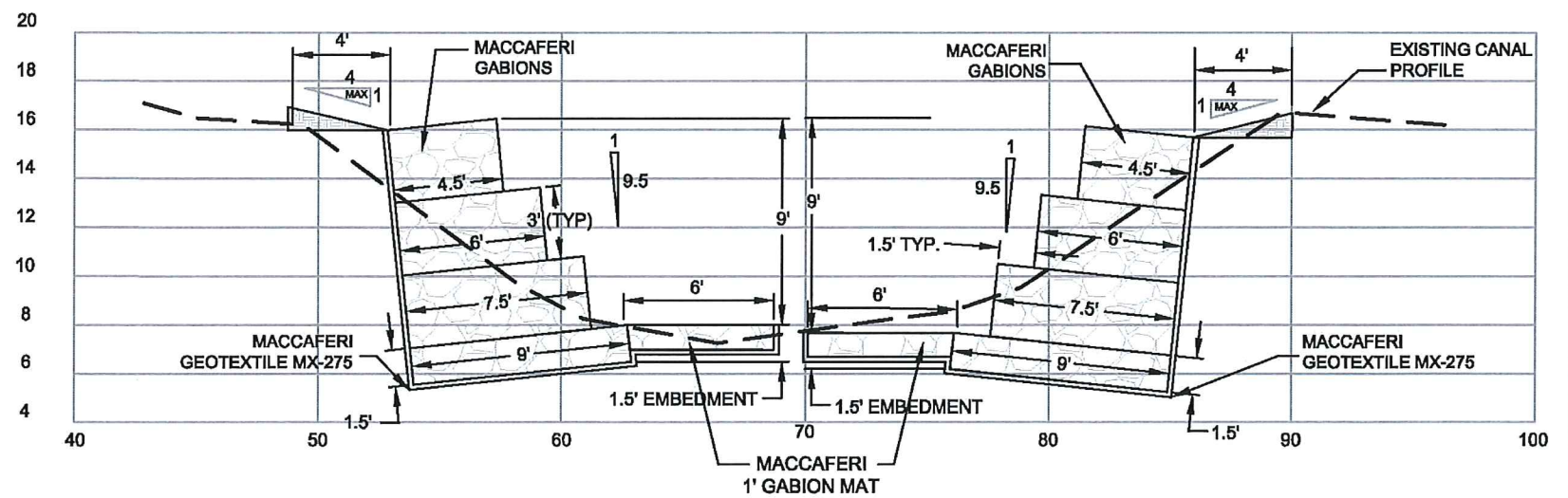
TYPICAL CANAL CROSS SECTION WITH GABIONS MACCAFERRI GABION WALL
