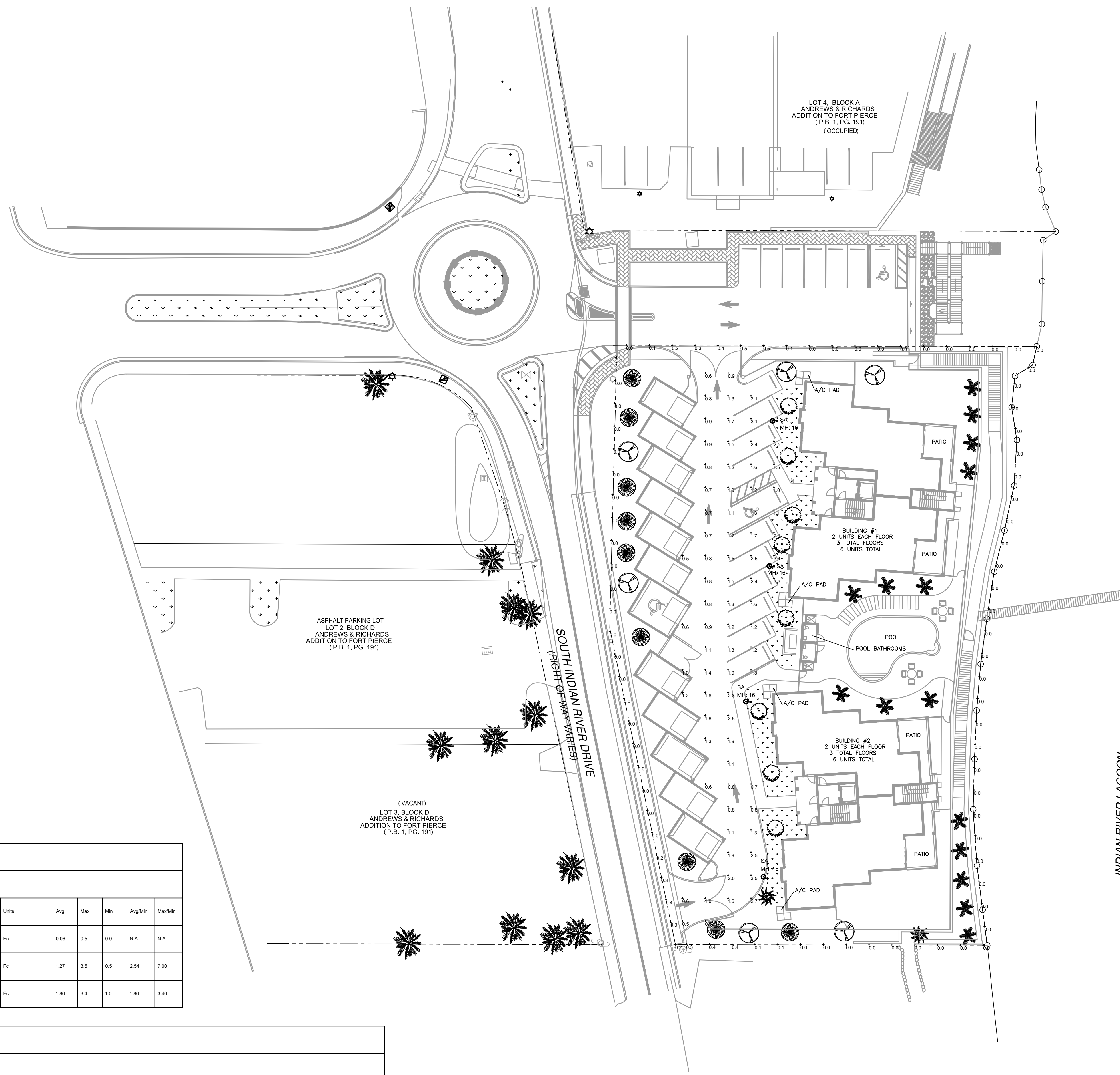
SITE PHOTOMETRIC PLAN 1/2"=1'-0" NORTH
