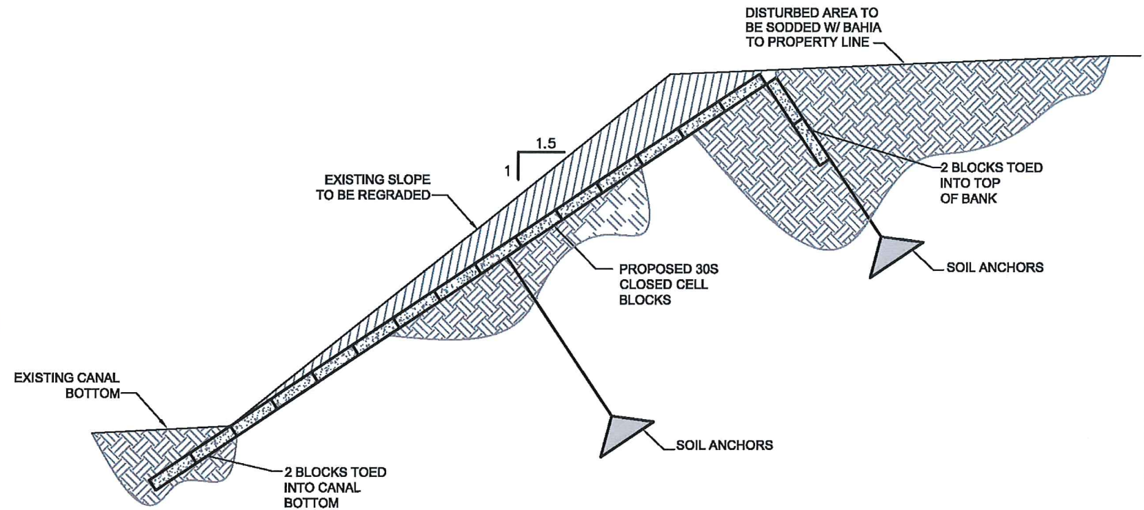
TYPICAL CANAL BANK STABILIZATION DETAIL
