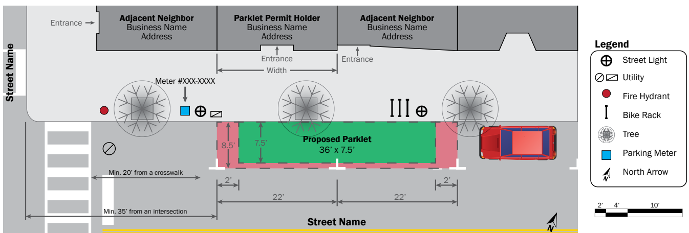
Figure 2 – Site Plan Requirements
