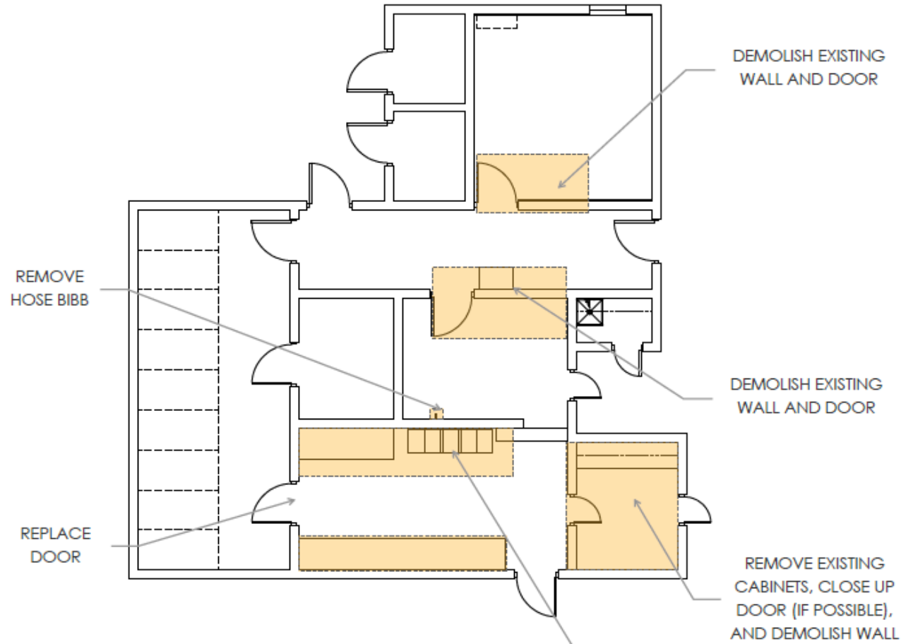
DEMOLITION DRAWING, 1/8" = 1'-0"
