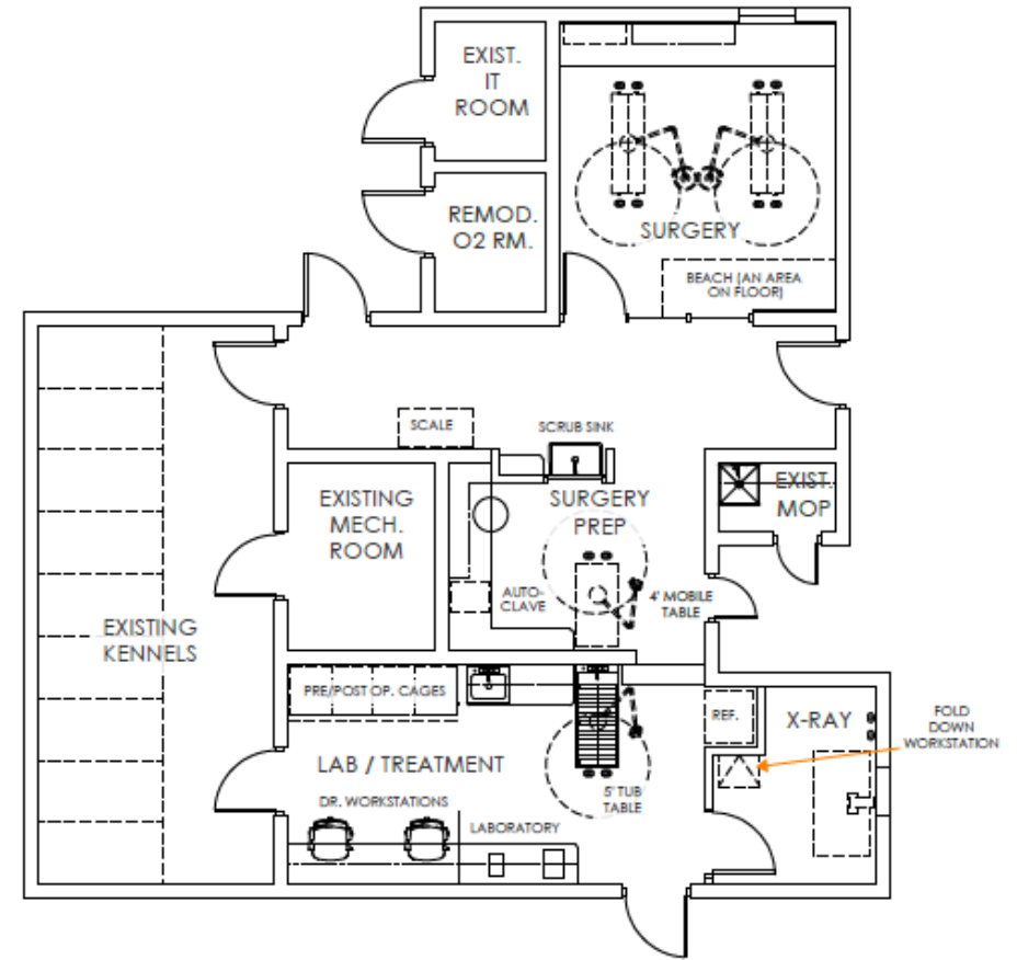
SURGERY FACILITY LAYOUT, 1/8" = 1'-0"
