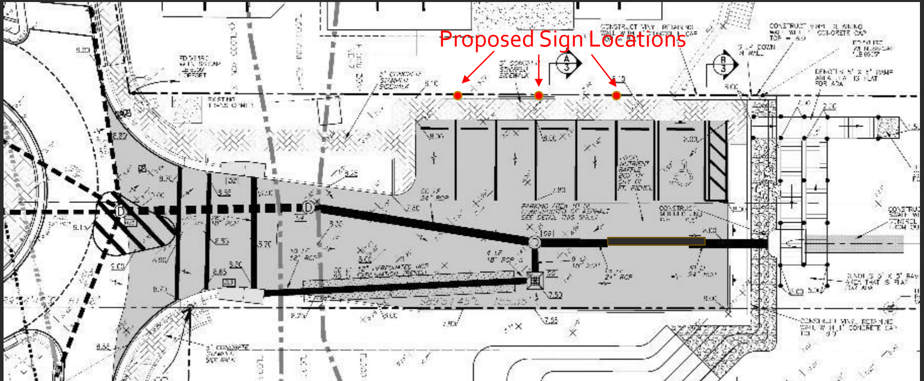
Existing Parking Layout
