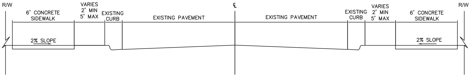
TYPICAL SECTION NEBRASKA AVENUE RIGHT-OF-WAY 80'
