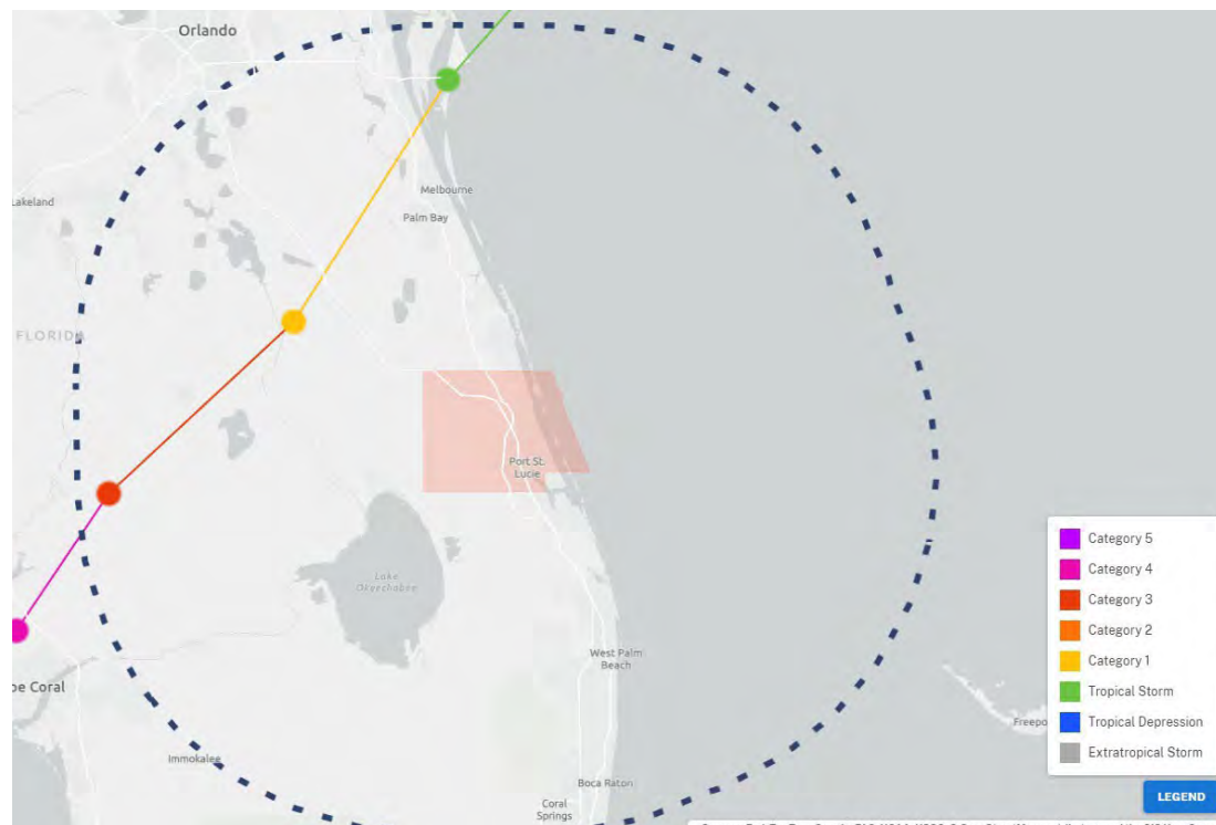
Figure 8-7. Hurricane Ian Storm Track
