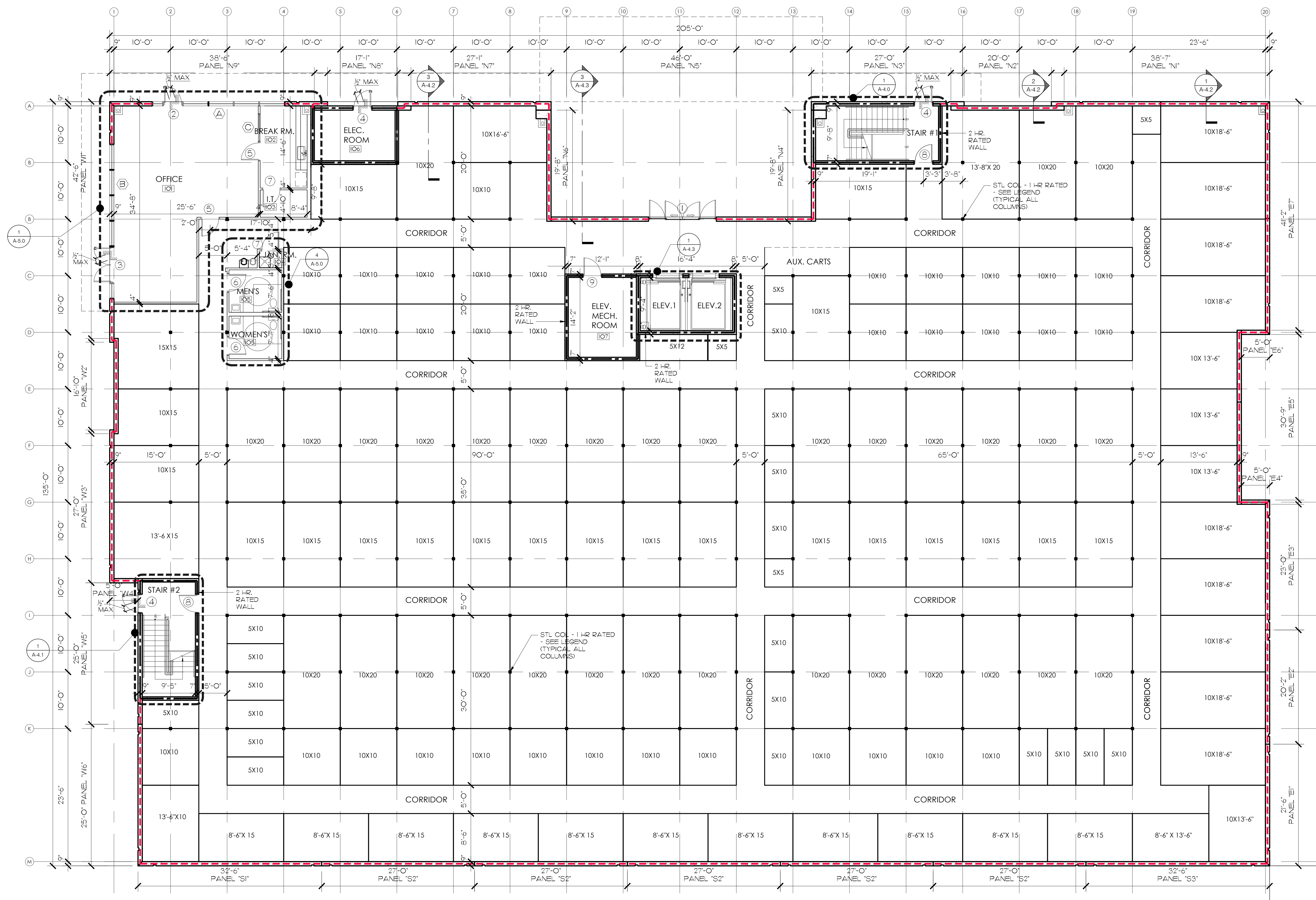
GROUND FLOOR PLAN SCALE: 1/8" = 1'-0"
