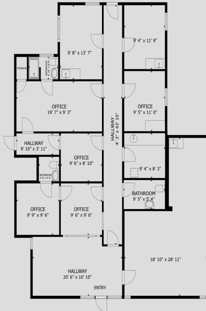
FLOOR PLAN
