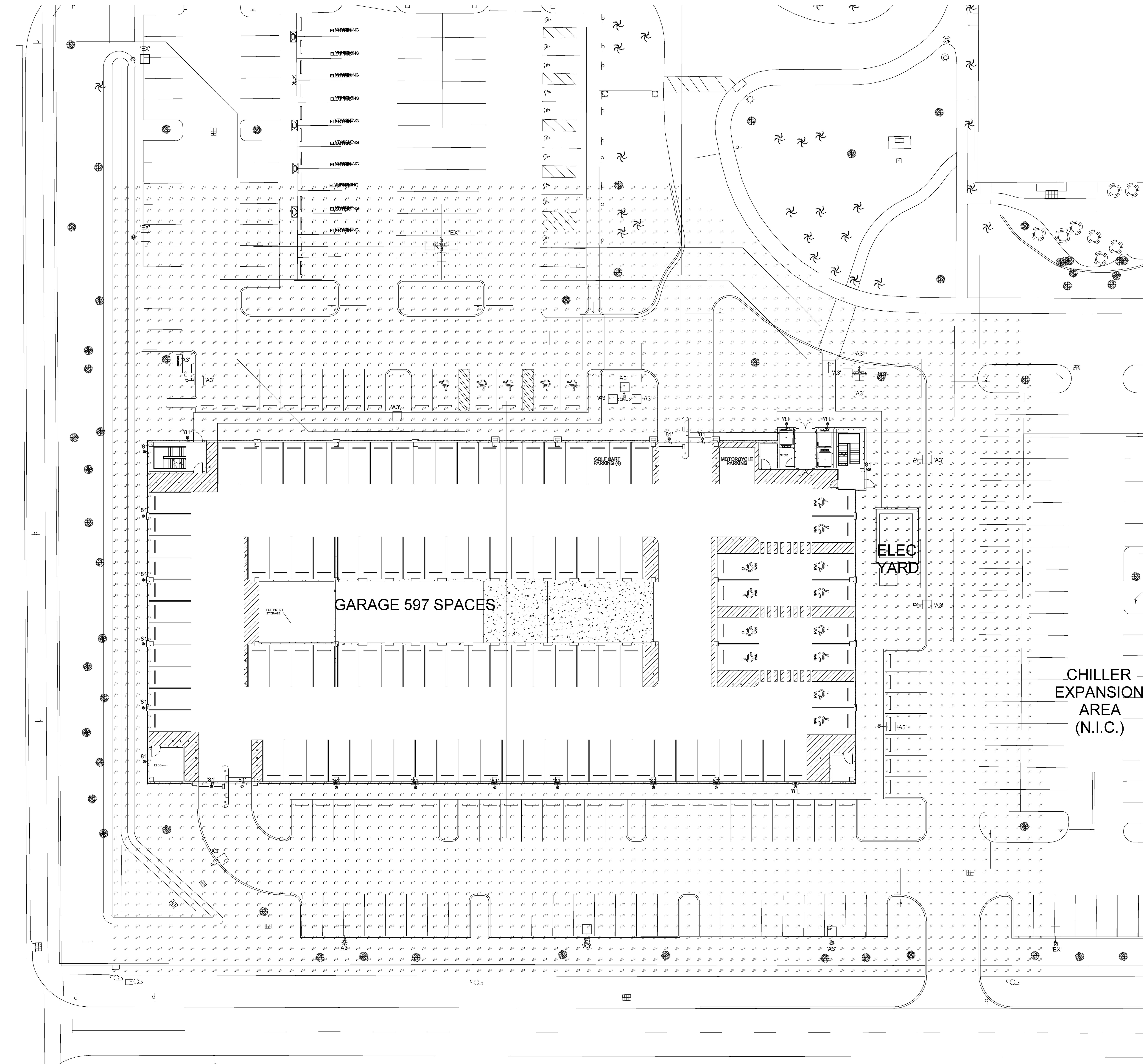
ELECTRICAL - SITE PHOTOMETRIC PLAN
