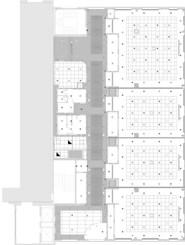
4TH FLOOR REFLECTED CEILING PLAN SCALE: 1/8" = 1'-0"
