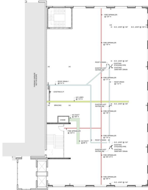
1 EXISTING 4TH FLOOR PLAN SCALE: 1/8" = 1'-0"
