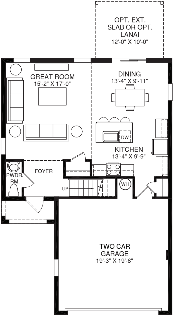
MAIN LEVEL
