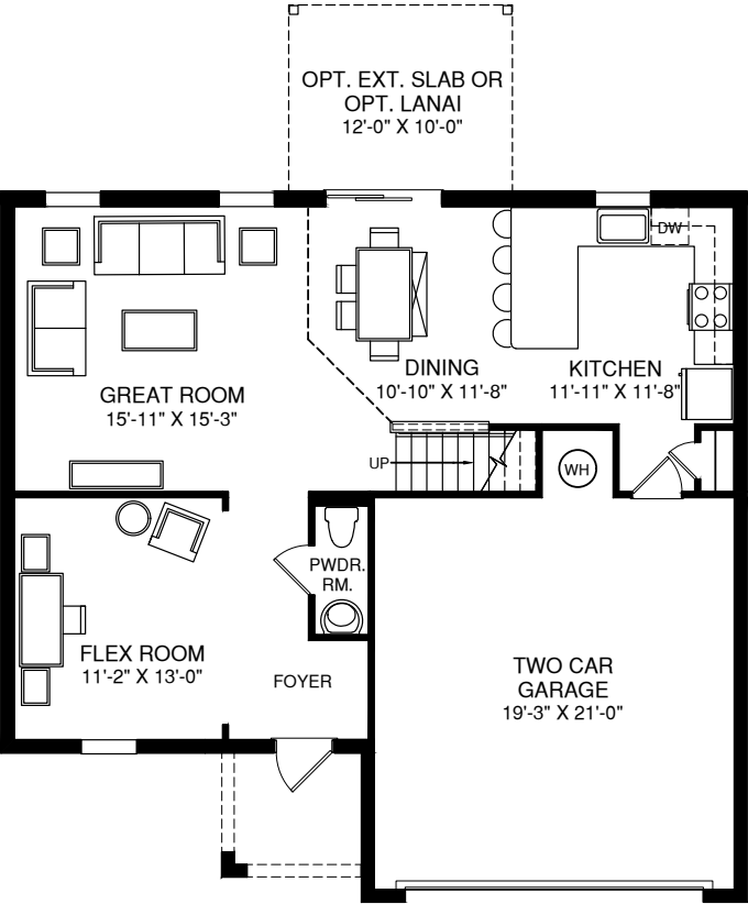
MAIN LEVEL
