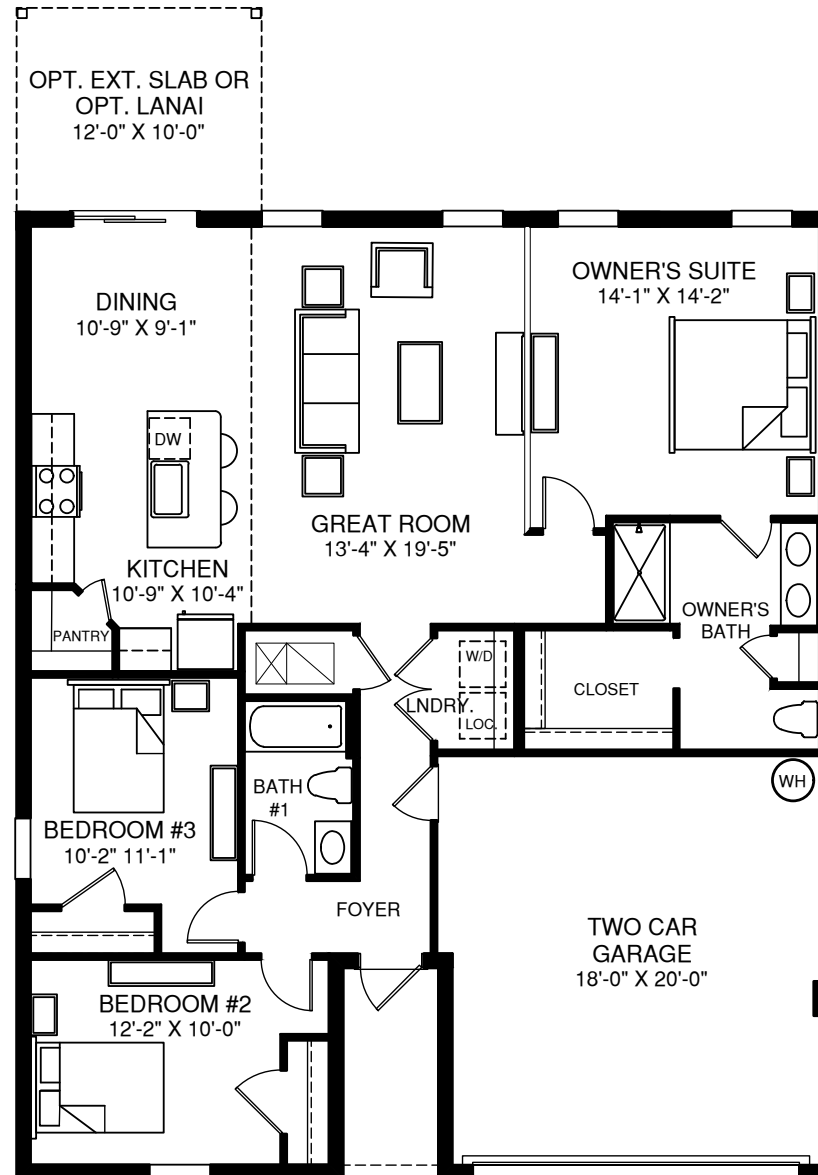
MAIN LEVEL
