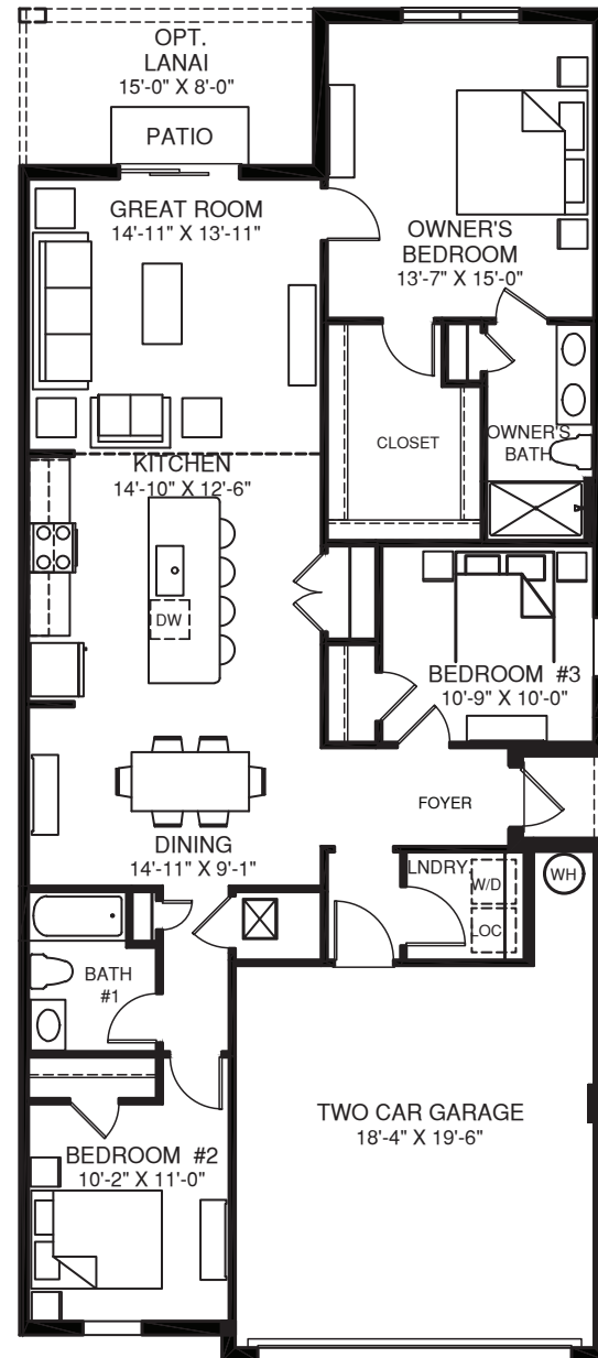
MAIN LEVEL
