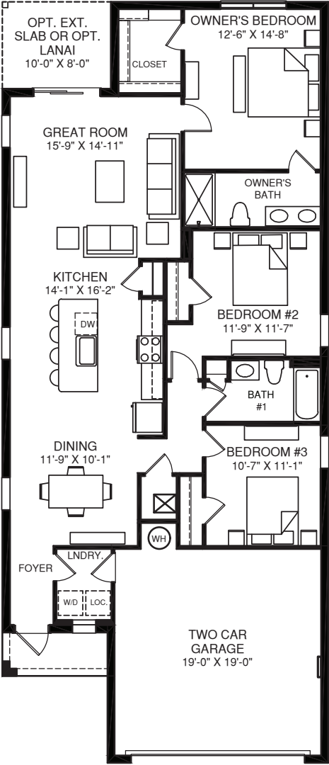
MAIN LEVEL
