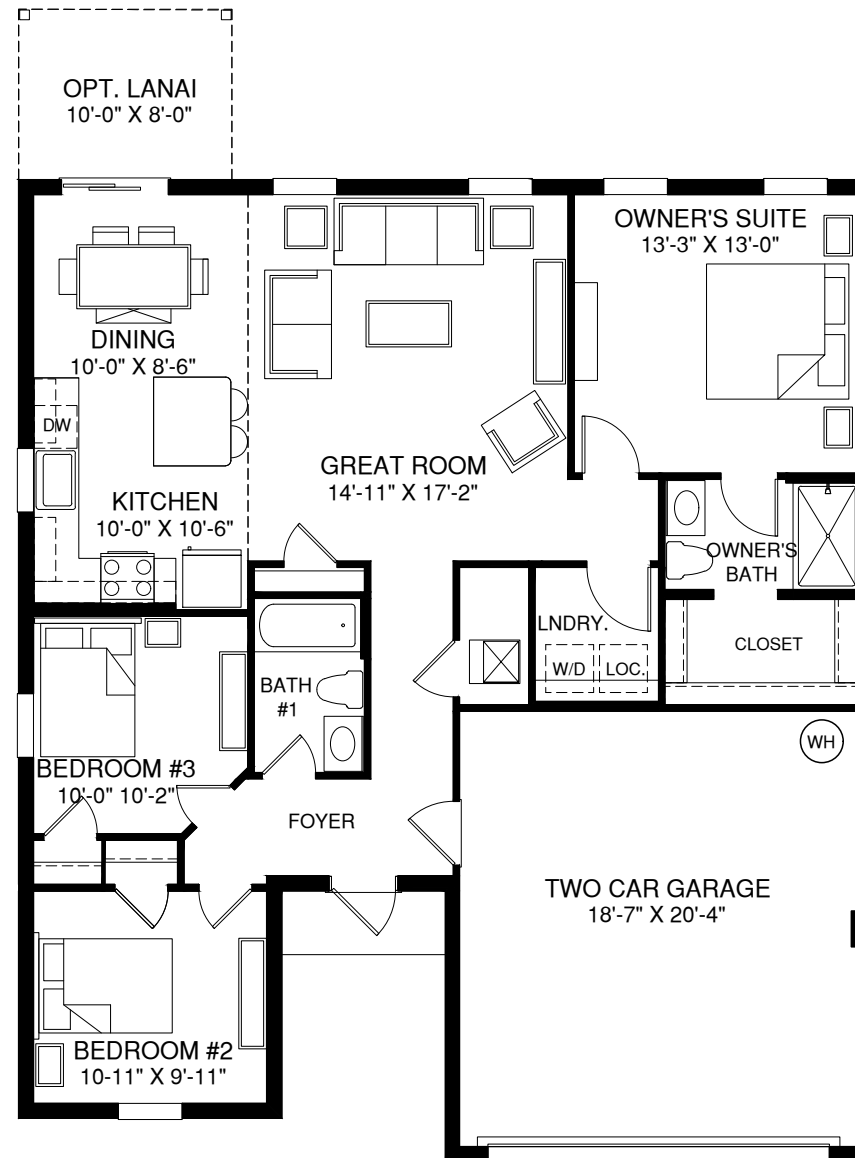
MAIN LEVEL
