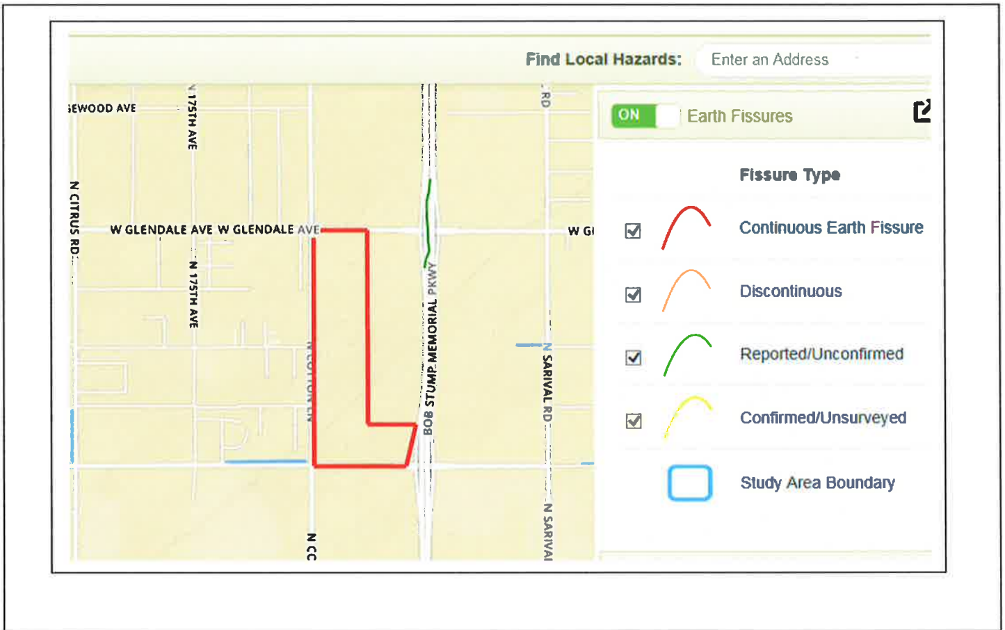
Figure #8 Subsidence/Fissures Arizona Geological Survey
