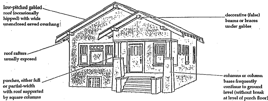
Figure 3: Craftsman Bungalow Building Style
