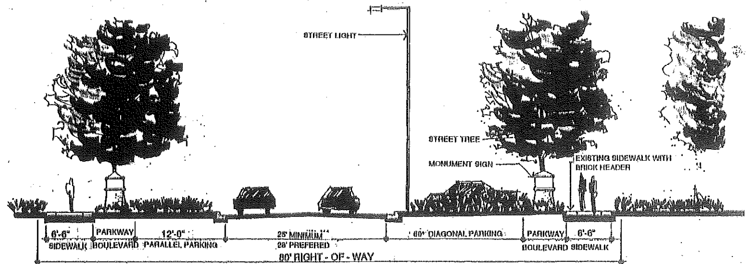
Figure 25; Typical Residential/Pedestrian Scale Entrance Monument Section
