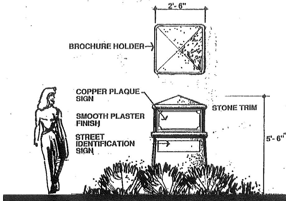
Figure 26; Pedestrian Scale Entrance Monument Sign
