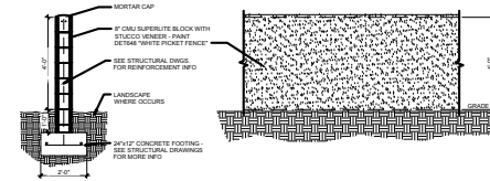
○ SITE SCREEN WALL - SECTION / ELEVATION NOT TO SCALE
